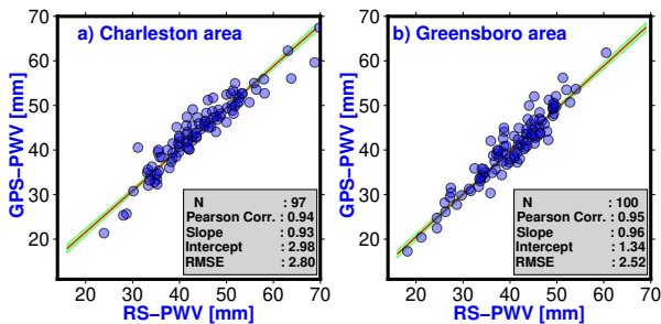
Fig. 2 Regression of PWV from GPS and radiosonde measurements at two stations; (a) The RS station at Charleston and GPS station SCFJ, and (b) the RS station at Greensboro and GPS station HIPT. The period covers from 24 August to 10 October 2018 at an interval of 12-hour temporal resolutions. The red line is the estimated linear regression and the green shadow that underlying in the red line is the 95% confidence interval. The number of data samples (N), Pearson correlation, slope, intercept and root mean square error (RMSE) are given in the legends.
