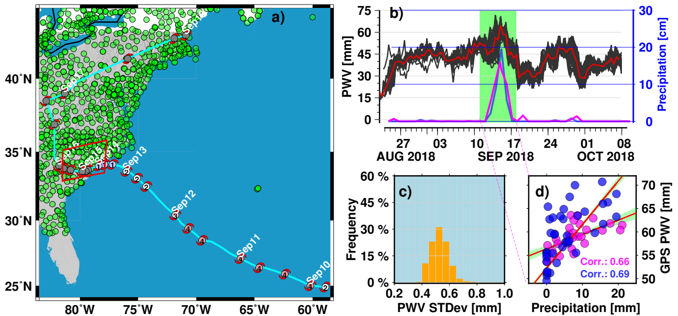
Fig. 1 a) Distribution of GPS stations shown as green circles. The cyan line is the actual path of Florence. The numbers on this line indicates the categories of the hurricane. b) Six-hours resolution stacked time series of GPS-PWV of individual GPS stations (black-lines) and averaged (red-line); stations within the red rectangle shown in panel map (a) are employed for a simple stacking. Superimposed are the daily accumulated GPM/IMERG (blue-line) and TRMM (magenta-line) precipitation time series. The light-green shaded region illustrates the periods where Florence shows a maximum change in GPS-PWV and precipitation. c) Histogram of the standard deviation (STDev) for GPS-PWV. The histogram was generated from the six-hour resolution stacked time series for the set of around 839 distributed stations for a period of two months in 2018. d) Scatter plot represents the regression between satellite-derived precipitation (i.e. GPM/IMERG is in blue-circles and TRMM is in magenta-circles) and GPS-PWV. The red line is the estimated linear regression and the green shadow is the 95% confidence interval. The regression is carried out with a three-hour resolution over the time periods of maximum change in GPS-PWV (i.e. 13–18 August 2018, i.e. the light-green shaded regions).
