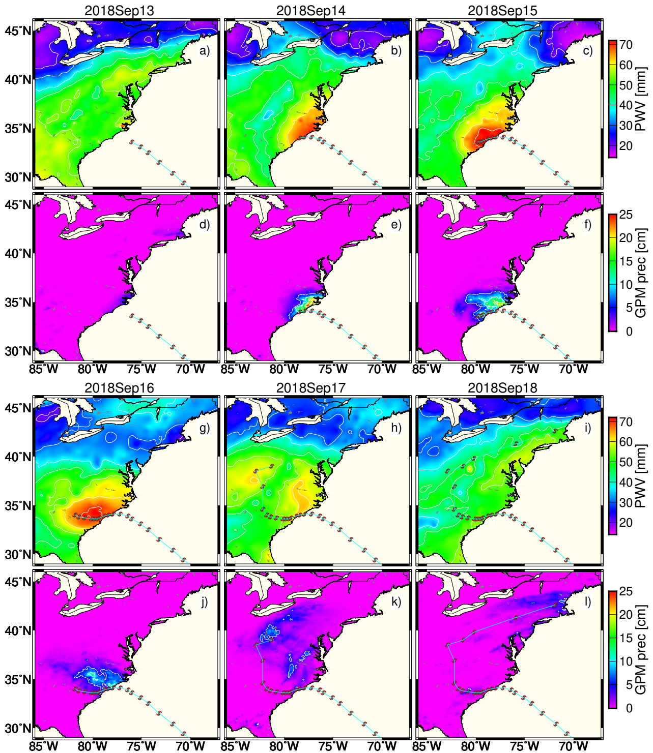
Fig. 3 Daily distribution maps for Hurricane Florence. GPS-PWV (first row a–c and third row g–i) and daily accumulated precipitation from GPM/IMERG (second row d–f and fourth row j–l) during Florence between 13 to 18 September 2018. The PWV and precipitation maps were created using the Generic Mapping Tools (GMT) by spherical surface spline gridding. The contour interval of the GPS-PWV is 7 mm, and the GPM/IMERG precipitation is 5 cm. The precipitation values are from GPM/IMERG. Florence’s path is plotted as the cyan line and the hurricane symbol as brown, respectively.
