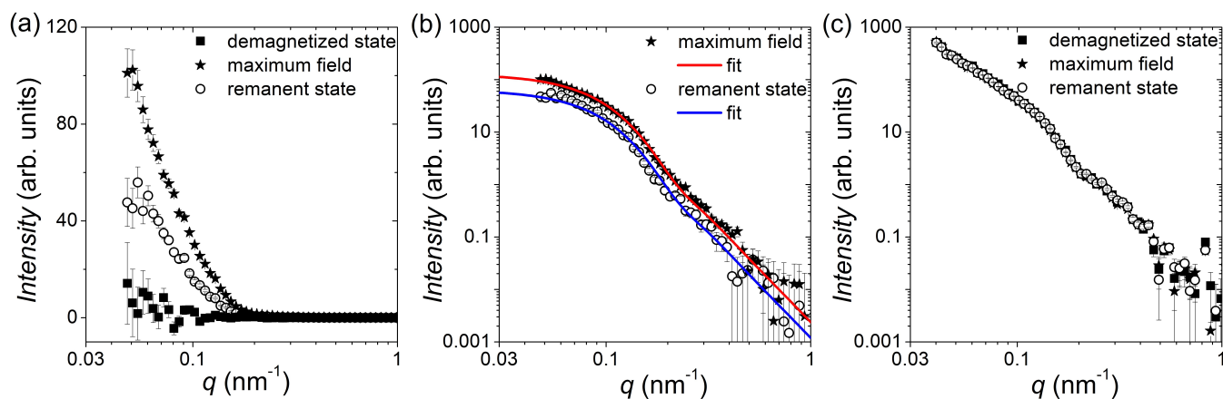
Fig. 5 (a) Nuclear-magnetic cross-term I_{\text{cross}}(q) detected at maximum field (i.e. magnetic saturation) and at zero field in the demagnetized state and remanent state, respectively (linear y-scale). (b) Fit of I_{\text{cross}}(q) in the saturated and remanent state with the spherical particle form factor (logarithmic y-scale). (c) Cross-section of I^+(q) parallel to \mathbf{H} in the saturated, demagnetized and remanent state. The scattering intensity of the bacteria without magnetosomes is subtracted.
