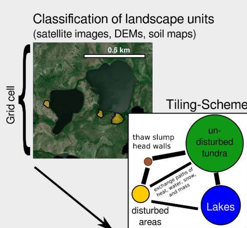
Conceptual illustration of the tiling scheme to simulate thaw slumps and their interaction with surrounding landscape units.
