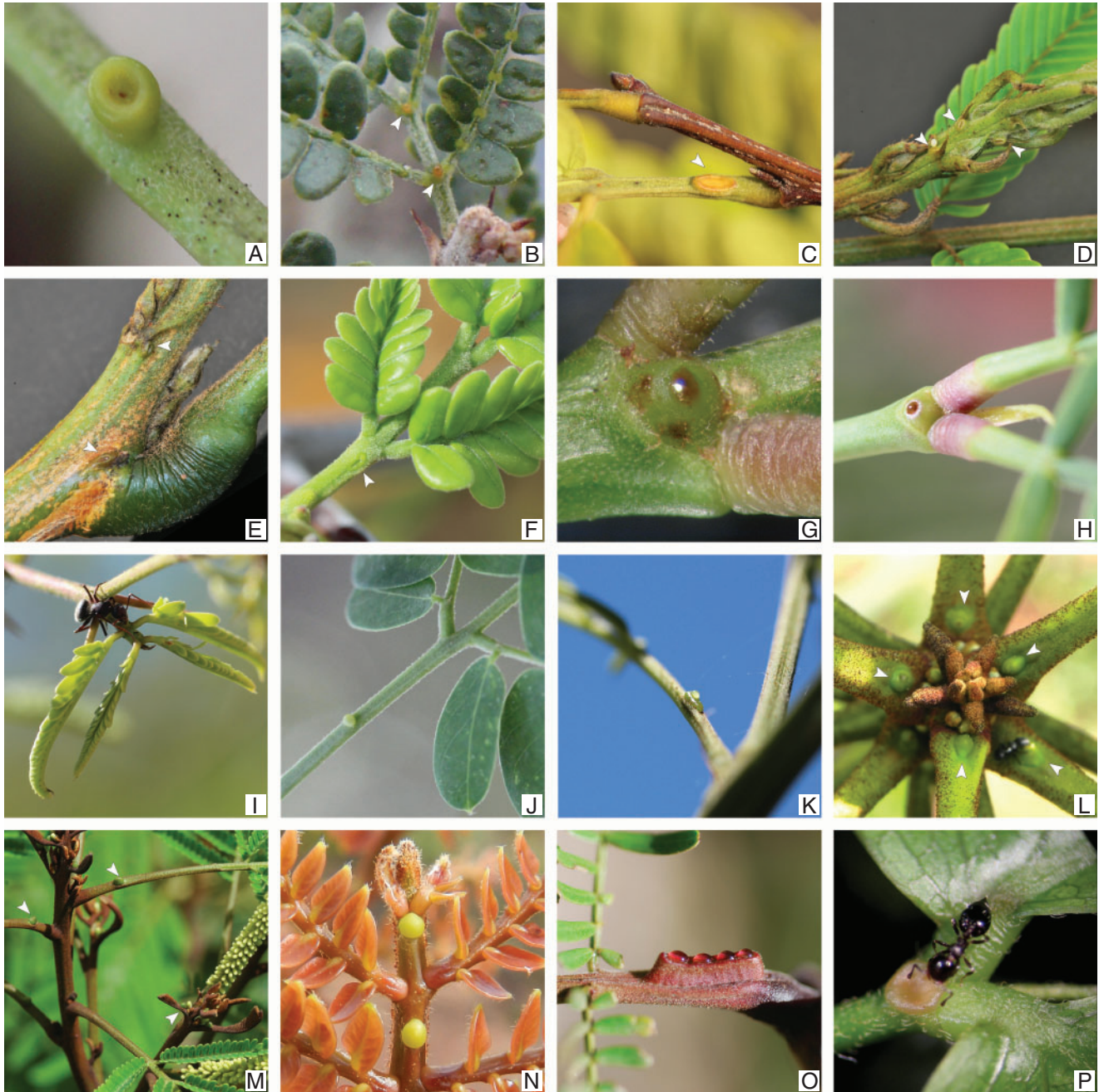
Fig. 13. Diversity of extrafloral nectaries (EFNs) in the Mimoid clade (Caesalpinioideae), Part 3 (genera M–Z). Arrowheads indicate positions of EFNs. All EFNs are parenchymatic and elevated. A. Mimosa irrigua , petiole. B. Painteria elachistophylla , rachis. C. Parapiptadenia sp. indet., petiole. D, E. Pentaclethra macroloba , stem below stipule in leaf axil. F. Pityrocarpa moniliformis , petiole. G. Prosopis alba , rachis. H. Prosopis nigra , rachis. I. Prosopis sp. indet., rachis. J. Pseudopiptadenia sp. indet., petiole. K. Senegalia bonariensis , petiole. L. Stryphnodendron adstringens , petiole. M. Stryphnodendron pulcherrimum , petiole. N. Stryphnodendron rotundifolium , rachis of young developing leaf. O. Vachellia collinsii , petiole. P. Zygia morongii , rachis. Photos: João Paulo Basso-Alves (D, E), Thais Cury de Barros (L), Martin Heil (O) and Erik Koenen (N).
