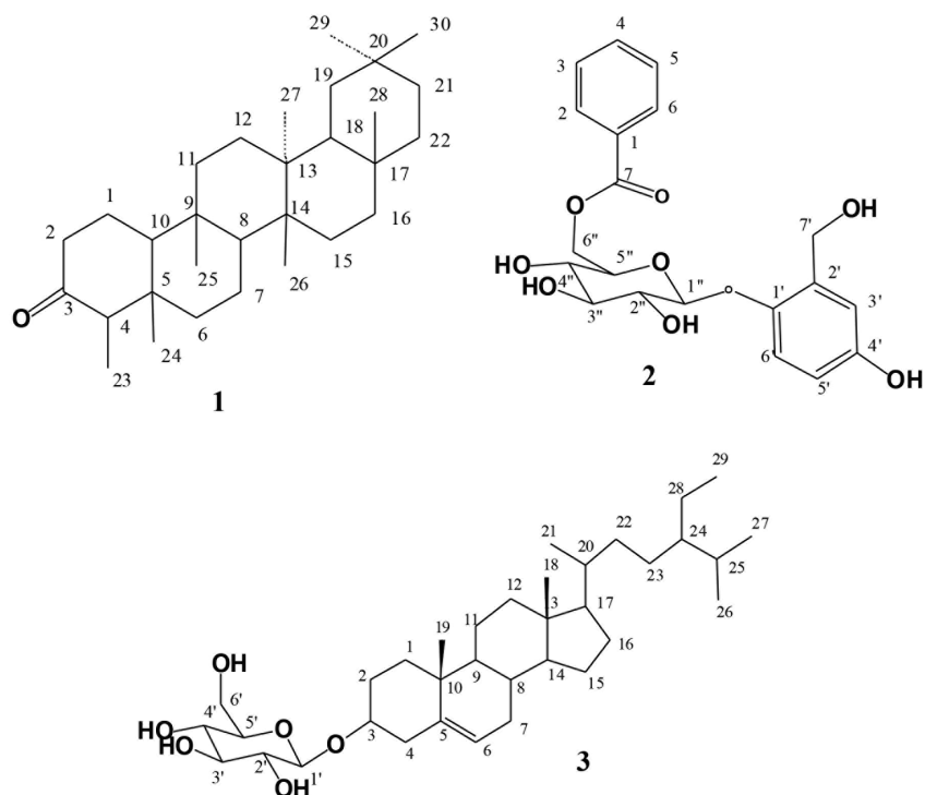
FIGURE 1. Structure of compound 1-3
