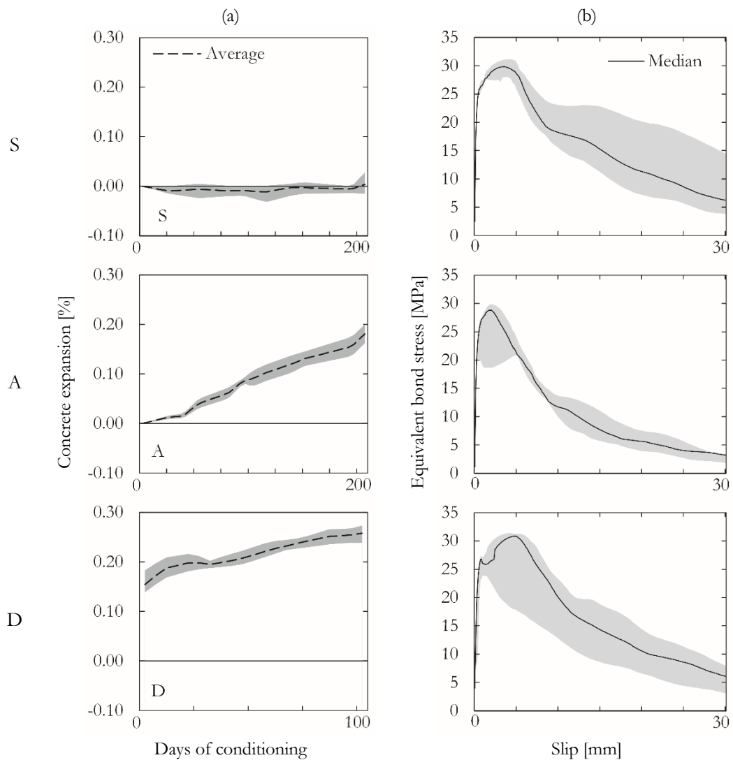
FIGURE 2: (a) Progression of the concrete expansion measured perpendicularly to the bar axis and (b) bond stress according to the epoxy bonded bar loaded end slip. The shade in graphs (a) and (b) marks out the maximum and minimum expansions and bond stresses, respectively.
