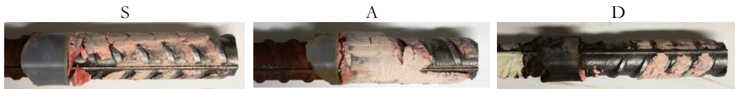
FIGURE 4: Typical epoxy bonded anchors after pullout.
