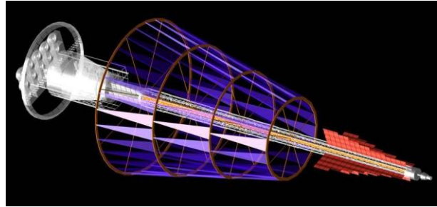
Fig. 1. Top - MARS-INPPS sub-systems with iBOSS building blocks. Bottom - first view of re-designed MARS-INPPS (for flight to Mars and Europa moon between 2025 – 2035) also contains about 15 – 20 iBOSS building blocks (see [1] to [6]).
