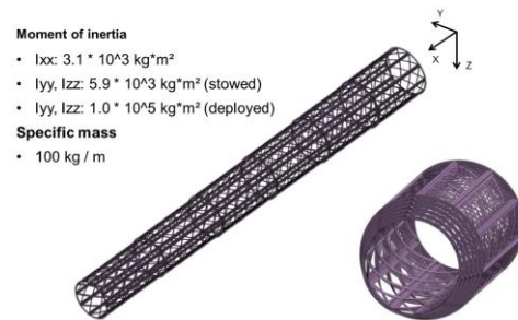
Fig. 3. Telescopic Grid Structure in deployed (left: 3 m diameter, 27 m length) and stowed (right: 3 m diameter, 4.5 m length) configuration.
