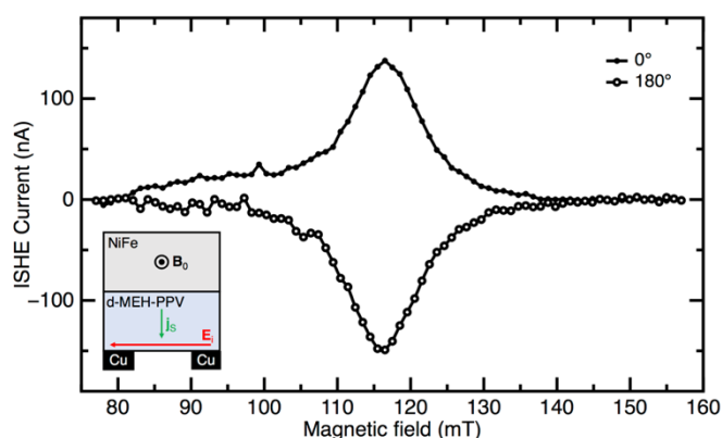
Figure 5 - Pulsed inverse spin-Hall (ISHE) response as a function of magnetic field, measured for opposing in-plane magnetic field orientations (0° and 180°). In brief, a spin current is generated in the organic semiconductor by the ferromagnetic resonance driven in the NiFe top contact. The inset shows a sketch of the device, consisting of a layer of d-MEHPPV on top of Cu electrodes, and covered with a NiFe film. An electric field E_i is generated between the two Cu electrodes and the orthogonal current j_s due to the ISHE is measured. The relative orientations of the static magnetic field, the injected spin current, and the resulting electromotive force on the charges are described in Sun et al. 23 The ISHE provides a metric for the strength of spin-orbit coupling in the semiconductor material.
