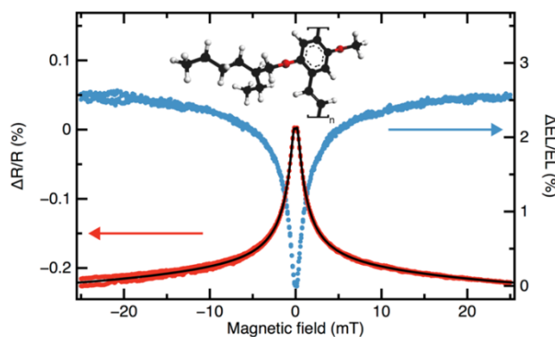
Figure 1 - Magnetoresistance (red) and magneto-electroluminescence (magnetoEL, blue) of OLEDs made of d-MEHPPV, along with a least-squares fit to the model described in Joshi et al. 12 (black line). Note that the measurements were performed under constant current to minimize the impact of conductivity changes on EL. The chemical structure of poly[2-(2-ethylhexyloxy- d 17 )-5-methoxy- d 3 -1,4-phenylenevinylene- d 4 ] (d-MEHPPV) is shown in the inset.
