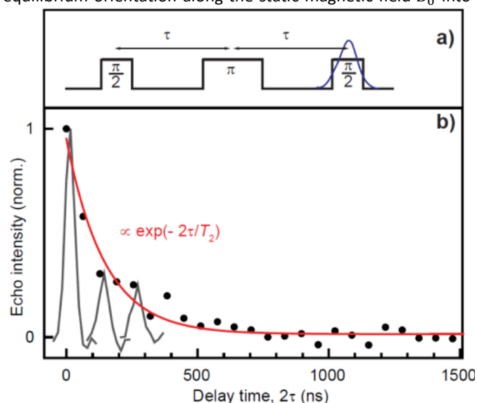
Figure 3 - Determination of the spin dephasing time T_2 in d-MEHPPV by an electrically detected Hahn echo measurement. 1,14,20-22 (a) Illustration of the modified Hahn echo pulse sequence for electrical detection: \pi/2 - \tau - \pi - \tau - \pi/2 . The final \pi/2 -pulse is not part of the conventional Hahn echo pulse sequence and serves to project the rephased spin echo onto a field axis parallel to the external field to enable electrical detection through a current measurement. The length of a \pi -pulse in these experiments was 32 ns. (b) Plots of the current-detected echo amplitude determined from individual measurements as a function of the delay time 2\tau . The red solid line represents a least-squares fit to an exponential decay time T_2 . Three examples of measured current echoes are superimposed such that their echo maxima overlap with the data point of the corresponding values of 2\tau (grey curves).
