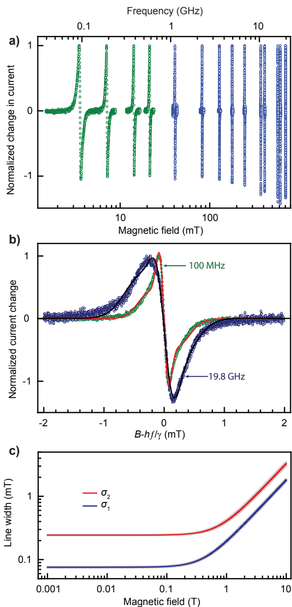
Figure 2 - Multi-frequency analysis of d-MEHPPV OLED devices at microwave frequencies below 20 GHz. 2,3,6,9,35 (a) Measured resonance lines normalized to the maximal current amplitude. (b) Comparison of the measured spectra at the lowest (100 MHz) and highest (19.8 GHz) frequencies, with the magnetic field axis normalized to the resonance field. The solid line represents the result of a global fit of all spectra obtained at all applied frequencies. (c) Variation of the root-mean-square resonance line widths of electron (red) and hole (blue) spins, as a function of the applied magnetic field (i.e., the excitation frequency). The displayed functions are the result of the numerical multi-frequency line-shape analysis of the data shown in (a) and (b), and the narrow grey shaded areas around the red and blue plots indicate the uncertainties in the line width obtained from a bootstrap analysis as described in Joshi et al. 3
