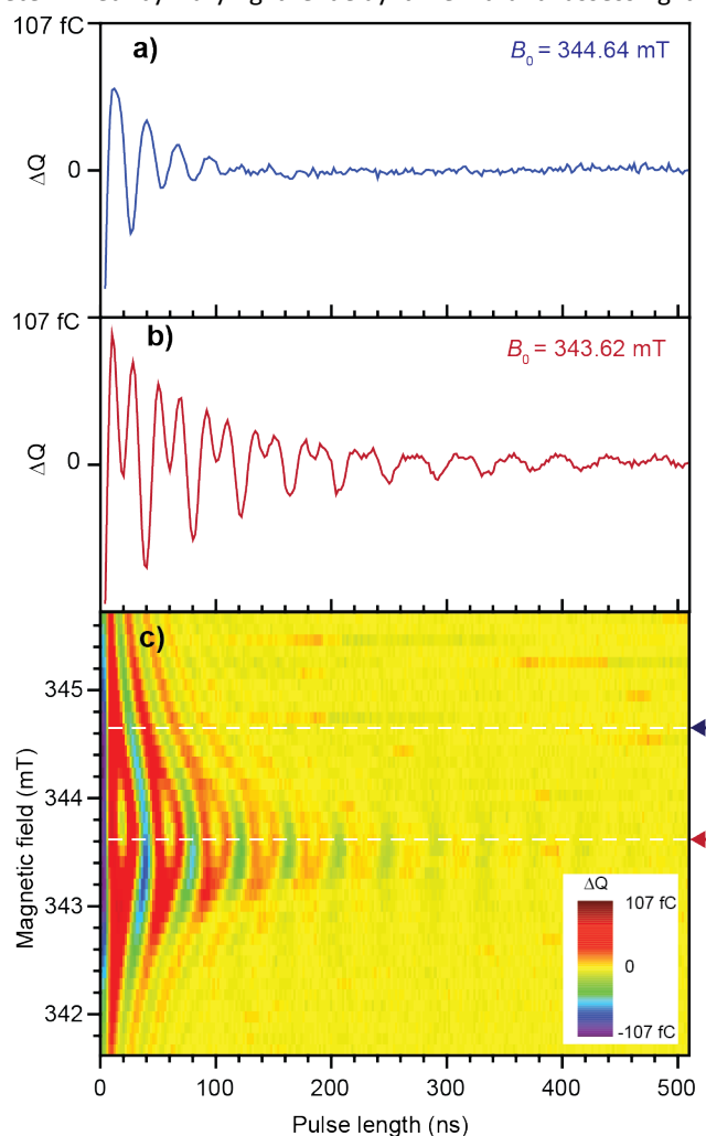
Figure 4 - Electrically detected charge-carrier spin-Rabi oscillations and evidence for spin-beating in d-MEHPPV OLEDs in a static magnetic field range close to the electron paramagnetic resonance condition under application of a \sim 9.7 GHz radiation pulse (i.e., at X-band). (a) Integration of the device current change from its steady-state value (i.e., the charge \Delta Q ) as a function of the length of the applied MW pulse for an arbitrary, slightly off-magnetic resonance magnetic field ( B_0 = 344.64 mT). The oscillation of the charge signal with pulse duration is due to a coherently driven Rabi nutation between the eigenstates of the spin pairs. (b) Data recorded from an experiment similar to (a) with identical experimental conditions, except for the static magnetic field, which is set to the resonance maximum ( B_0 = 343.62 mT). Here, both charge carrier spins within the charge carrier pair nutate with time, so that a quantum beat (spin-locking) signal at the second harmonic frequency of the fundamental oscillation period emerges. (c) Contour plot of the Rabi oscillations shown in (a) and (b) as a function of the external magnetic field, showing the detuning from magnetic resonance. The blue and red arrows indicate the magnetic fields that correspond to the conditions of the data in panels (a) and (b).
