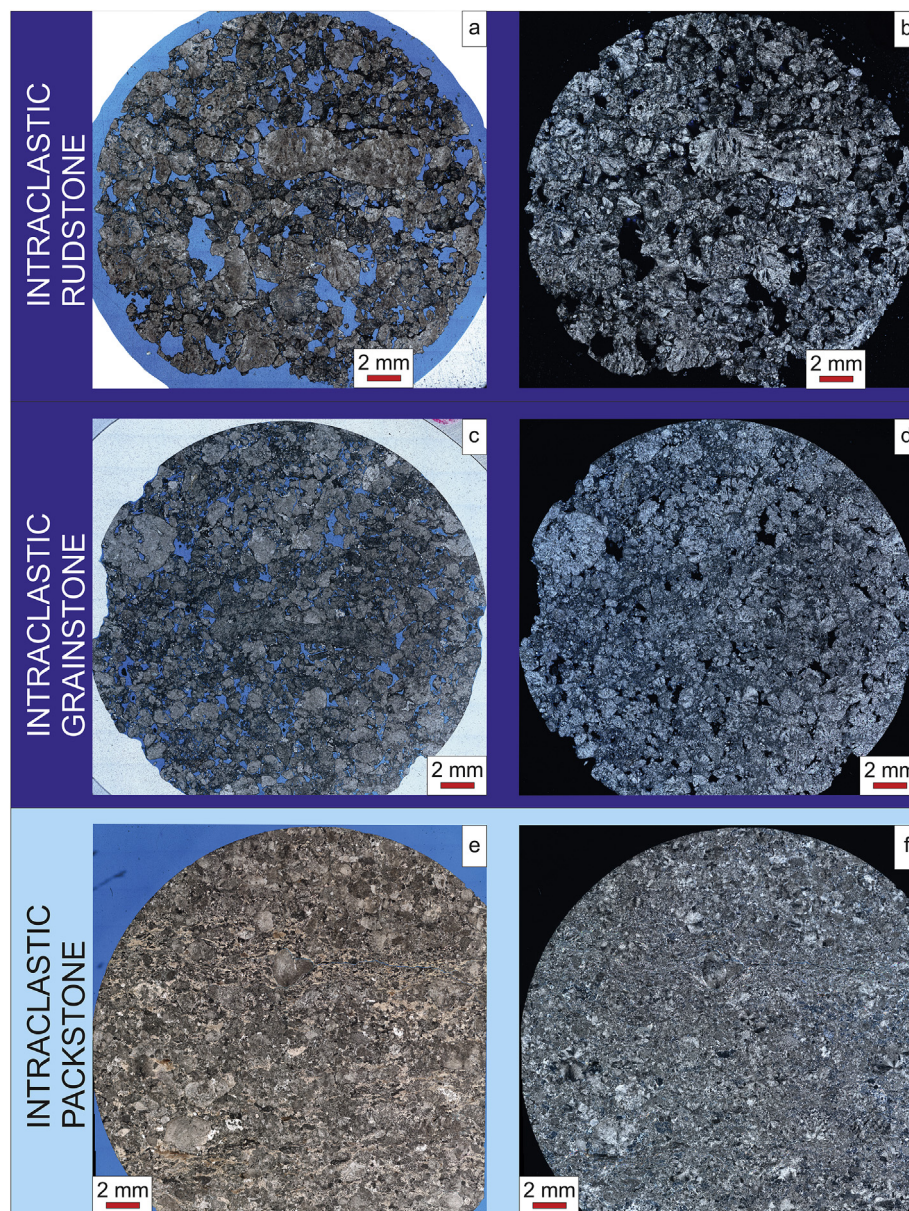
Fig. 9. Classification for reworked facies: a) and b) intracrystalline rudstone with inter-particle porosity; c) and d) intracrystalline grainstone with inter-particle porosity; e) and f) intracrystalline packstone. All image pairs are PPL and XP.
