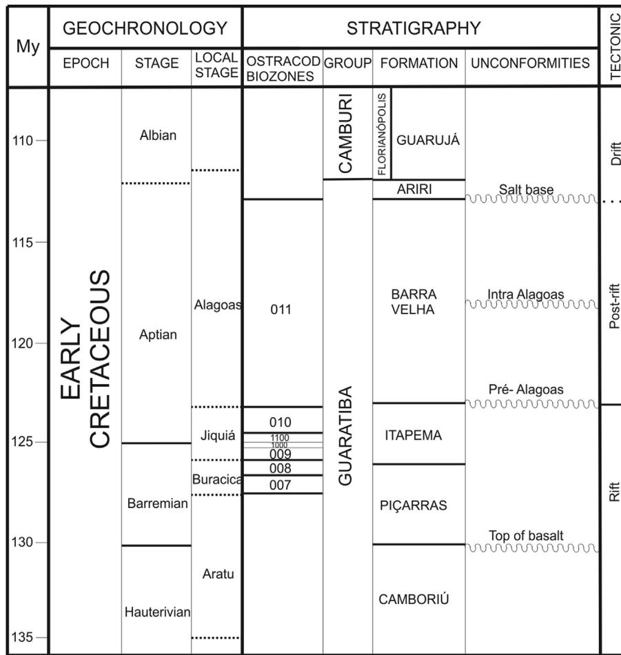
Fig. 2. Lower Cretaceous stratigraphic chart for the Santos Basin (adapted from Moreira et al., 2007) and ostracod biozones (modified from Pietzsch et al., 2018). The present study focusses on the Barra Velha Formation, which is bounded by the Pre-Alagoas and Salt Base unconformities and separated into the Lower and Upper Barra Velha Formation by the Intra-Alagoas Unconformity. The Barra Vellha Formation was deposited during the Alagoas local stage, which is correlated to ostracod biozone 011 and broadly to the Aptian (Moreira et al., 2007).
