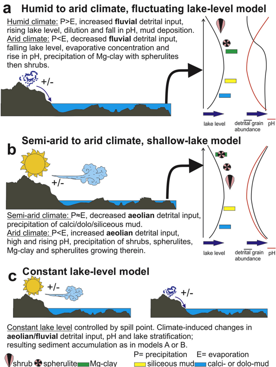
Fig. 20. Alternative conceptual models to explain temporal variations of detrital material within the Barra Velha Formation: a) Humid to arid climate, fluctuating lake-level model. b) Semi-arid to arid climate, shallow-lake model. c) Constant lake level controlled by spill point. Black arrows point at the stage of the model for the lake x-section.
