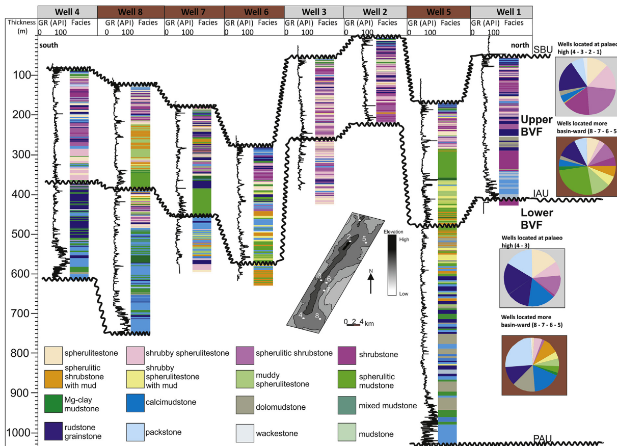
Fig. 12. Cross-section showing facies distribution for the 8 wells and the three main unconformities within the Barra Velha Formation. The distribution of facies shows a predominance of Mg-clay at wells drilled more basin-ward, whereas in-situ carbonate facies occur in the wells drilled on the palaeo-high. BVF = Barra Velha Formation, PAU = Pre-Alagoas Unconformity, IAU = Intra-Alagoas Unconformity, SBU = Salt Base Unconformity.
