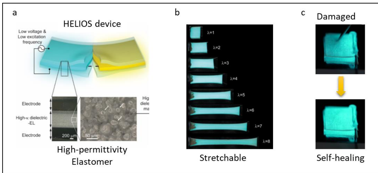
FIG. 1| Highly stretchable, high dielectric, self healing elastomer. a , illustration of the high permittivity material with embedded electroluminescent particles, sandwiched by ionic liquid-doped outer electrodes, forming the tri-layer HELIOS optoelectronic device. b , the HELIOS device can be stretched up to eight times its original length without breaking. c , the device can be damaged (here, pierced with a needle) and will self-heal, maintaining light output. Adapted from ref.2, SN.
