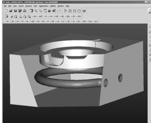
Figure15 - Conformal Cooling
