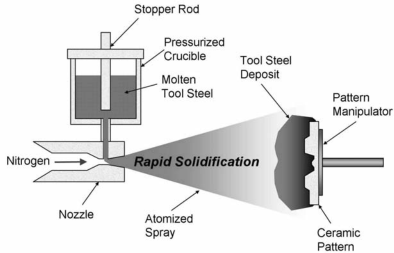
Figure 3 - Machine Process
