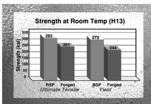
Figure 11 - H13 after Artificial Aging
