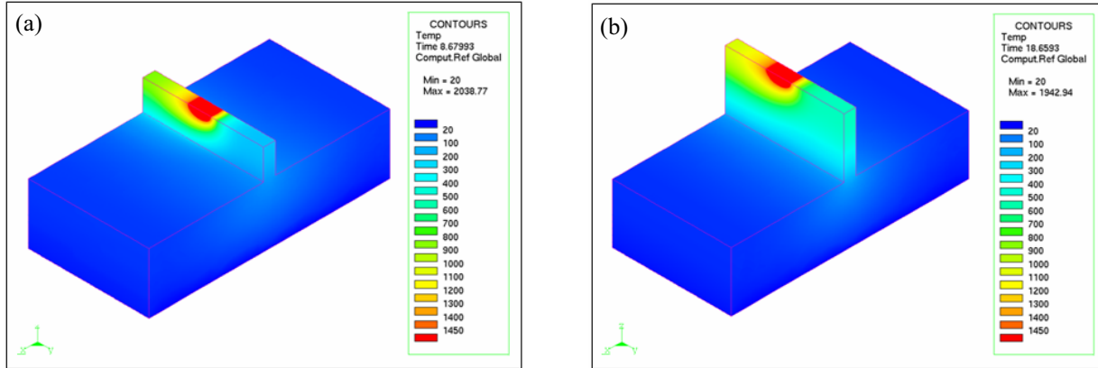
Figure 5 - Three dimensional temperature distributions when the laser beam moves to the center of (a) the 5 th layer, and (b) the 10 th layer of the deposited plate.
