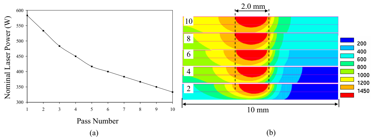
Figure 4 - (a) Nominal laser powers for each pass to achieve a steady molten pool size; (b) Molten pool size and shape when the laser beam moves to the center of the part for layers 2, 4, 6, 8 and 10. The average size of the molten pool is 2.0 mm. The molten pool size is determined by the melting temperature of SS410 (1450°C).
