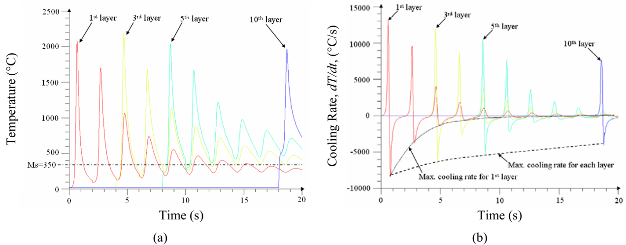
Figure 6 (a) Thermal cycles, and (b) Cooling rates for the mid-points of layers 1, 3, 5 of the built profile varies with time.
