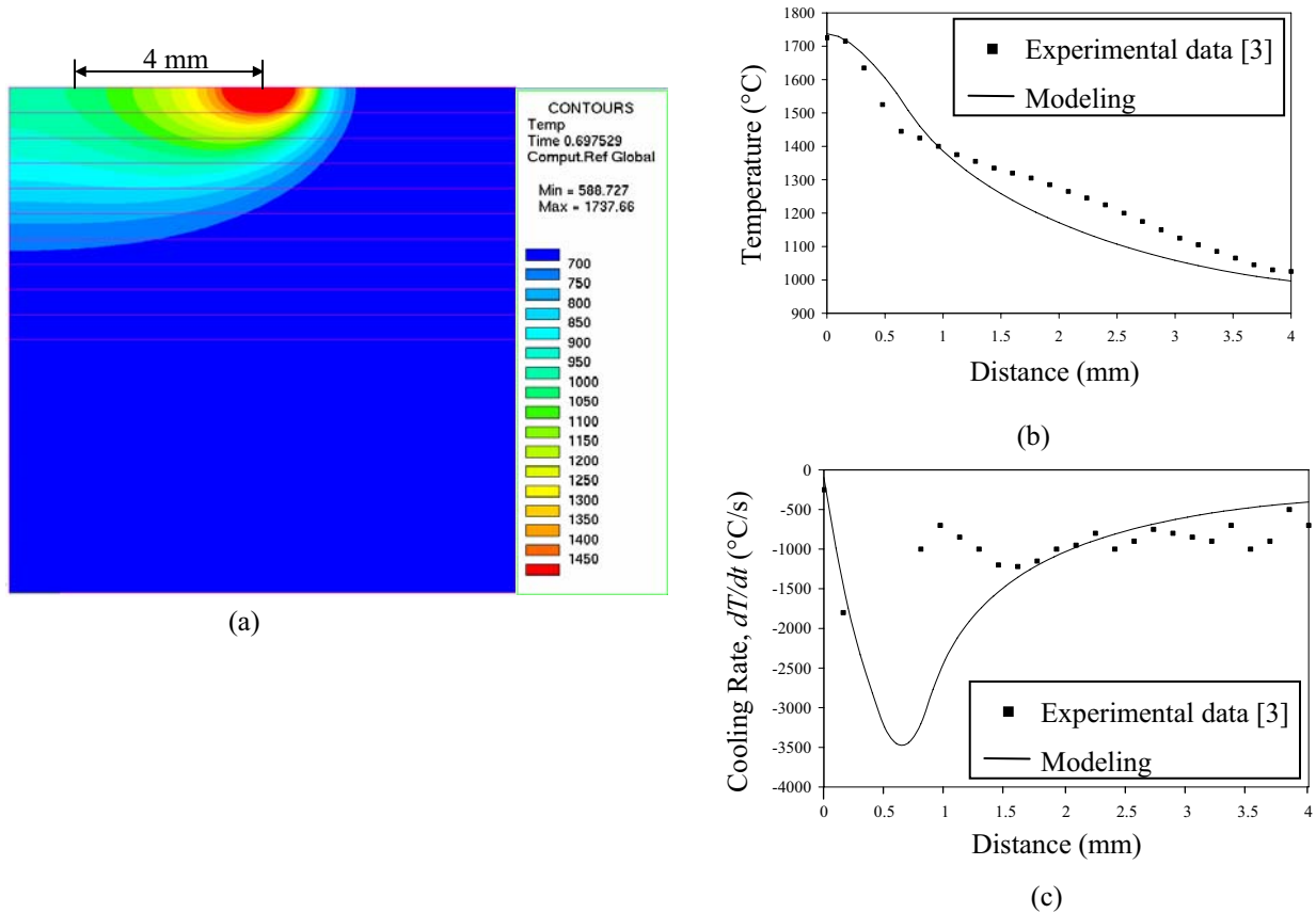
Figure 3 - (a) Calculated temperature distribution during deposition of SS410. (b) and (c): Model and experiment comparison of temperature profile (b) and cooling rate (c). The profiles are shown from the center of the molten pool along the travel direction of deposited part.
