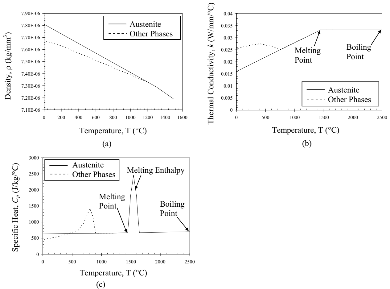
Figure 2 - Thermal properties used for SS410, (a) density, (b) thermal conductivity, (c) specific heat.
