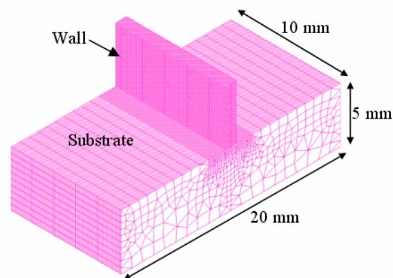
Figure 1 - Finite element mesh and geometry to simulate the LENS process for a 10 layer plate.
