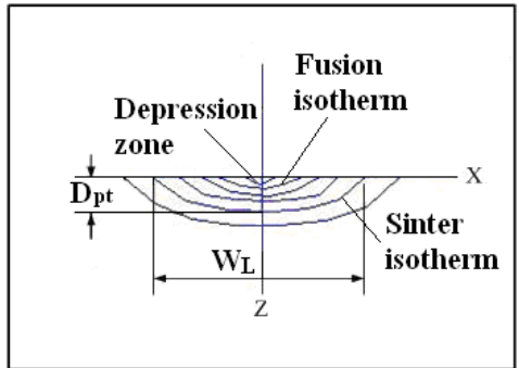
Fig. 2 Temperature distribution corresponding to the energy distribution of the Gaussian beam
