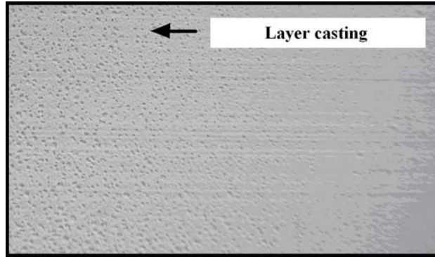
Fig. 2 Deterioration of the surface quality along the layer casting
