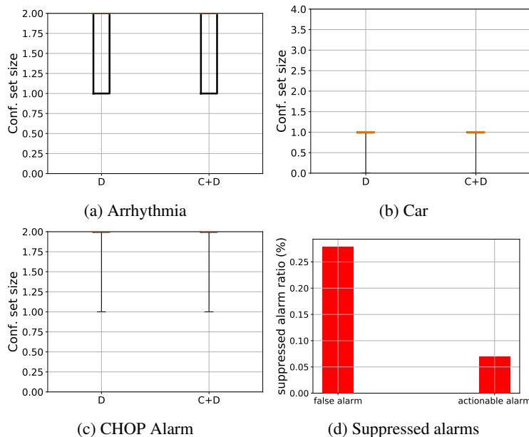
Figure 7: Confidence set sizes for three additional classification benchmarks: (a) the arrhythmia detection dataset (Guvendir et al., 1997); here, n = 90 , \epsilon = 0.1 , \delta = 0.05 , and the empirical confidence set error of our approach C + D is 0.0435, (b) the car evaluation dataset (Bohanec & Rajkovic, 1988); here, n = 345 , \epsilon = 0.05 , \delta = 10^{-5} , and the empirical confidence set error of our approach C + D is 0.0172, and (c) the CHOP alarm dataset (Bonafide et al., 2017); here, n = 1000 , \epsilon = 0.02 , \delta = 10^{-5} , and the empirical confidence set error of our approach C + D is 0.0159. (d) The fractions of actionable and false alarms with a confidence set \{0\} (i.e., only contains false alarm).
