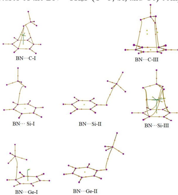
Figure 3 The AIM diagrams of the \sigma -hole tetrel bond complexes. Small dots refer to bond critical points.
