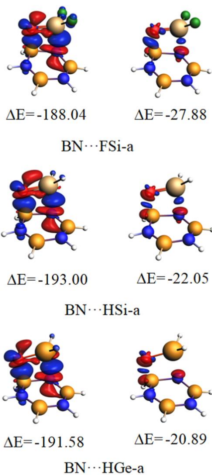
Figure 6 Plots of deformation densities of the pair-wise orbital interactions ( \Delta\rho ) in the a complexes of F_2SiO and H_2TO ( T=Si and Ge ) at the GGA-PBE-D3/TZ2P//MP2/aug-cc-pVTZ level. The associated orbital interaction energies are given in kcal/mol. The color code of the charge flow is red→blue and the isovalue for \Delta\rho is 0.005 au.
