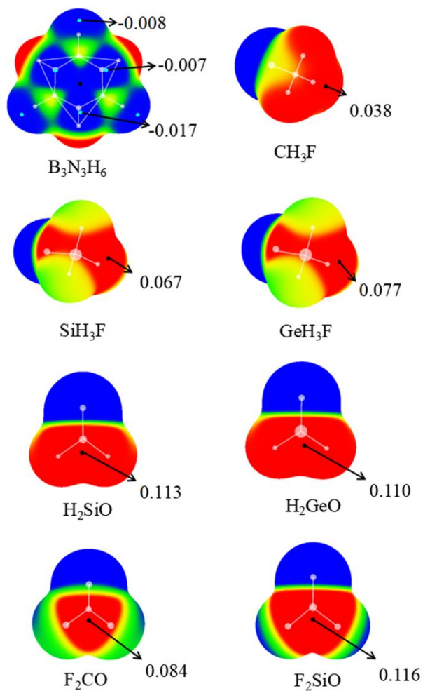
Figure 1 MEP diagrams of the monomers. Color ranges, in au, are: red, greater than 0.02; yellow, between 0.01 and 0.02, green, between 0 and 0.01; and blue, less than zero.
