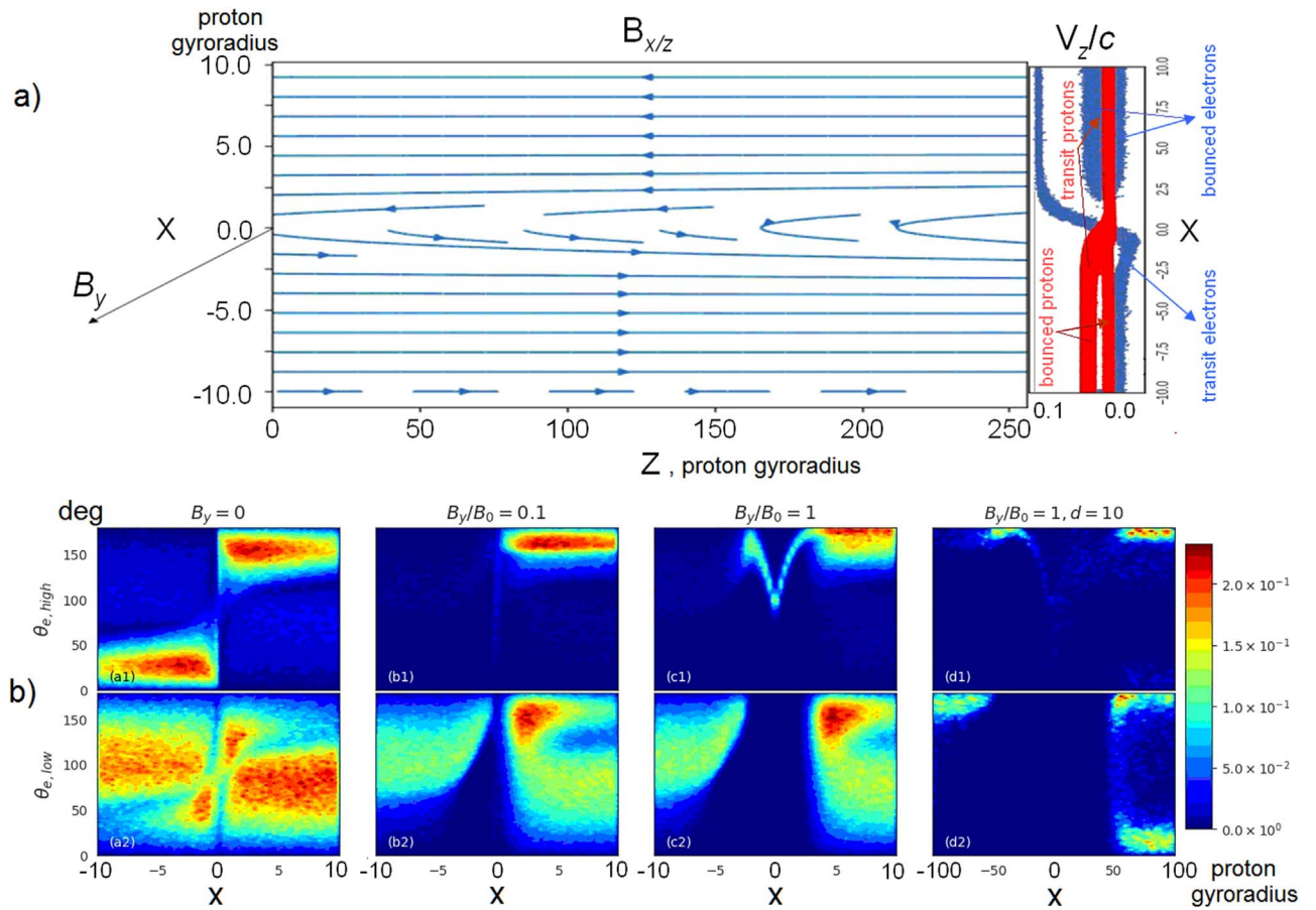
Figure 4. Model of the acceleration of solar wind electrons to suprathermal energies at the 3D RCS. (a) Topology of magnetic field lines in the vicinity of the single X-null point of the RCS (on the left), and example of 2.5D particle-in-cell simulations (3D by velocity V and 2D by coordinate) of particle trajectories for the strong guide field, B_y/B_0 = 1 (on the right). Bounced particles form clouds at the injection side with respect to the midplane, but more energetic transit particles are ejected into the opposite semiplane. (b) PADs for electrons with lower energy (bottom row) and higher energy (top row) for the guide field B_y of different strength: B_y/B_0 = 0 (first column, weak guide field), 0.1 (second column), and 1.0 (third column, strong guide field). RCS width d = 1.0 \rho_i (thin RCS) in the three columns ( B_0 = 10^{-9} T). The fourth column is given for comparison under the conditions of thicker RCS and strong guide field ( B_y/B_0 = 1 , d = 10 \rho_i ).
