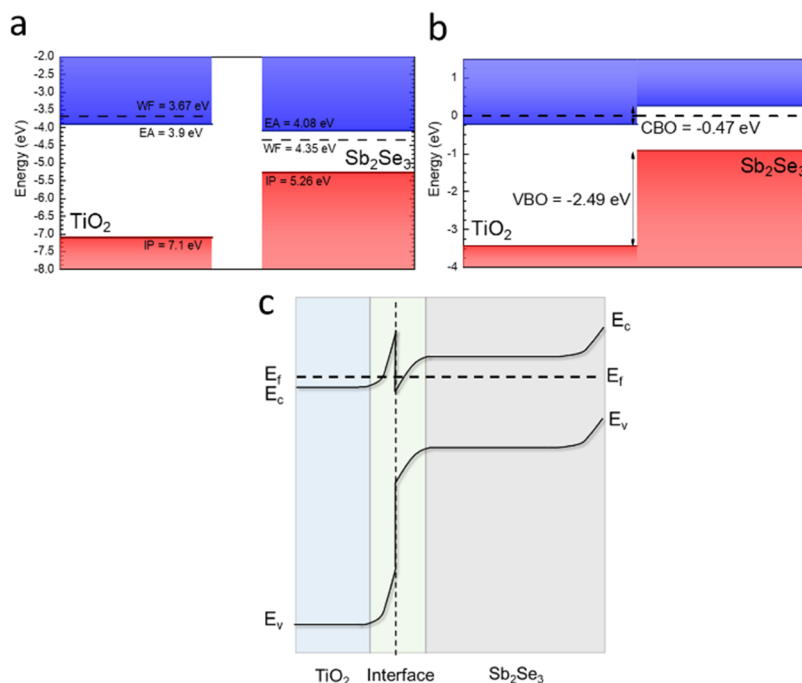
Figure 6. (a) \text{TiO}_2 and \text{Sb}_2\text{Se}_3 energy level positions determined from XPS analysis showing electron affinity (EA), work function (WF), and ionization potential (IP) of each material, (b) band alignment of the \text{TiO}_2/\text{Sb}_2\text{Se}_3 interface, and (c) proposed band structure of \text{TiO}_2/\text{Sb}_2\text{Se}_3 .
