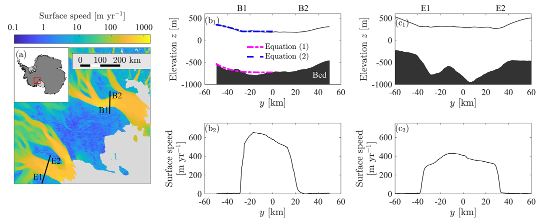
Figure 1. Examples of ice stream profiles. Panel a shows velocity map of the Siple Coast, with the location of the two profiles in panels b and c marked with black lines. Gray shading indicates the Ross ice shelf. Panel b_1 shows surface elevation and bed across Whillans ice stream, and panel b_2 shows the surface velocity across the same profile. Panel c_1 shows surface elevation and bed across MacAyeal ice stream, and panel c_2 shows the surface velocity across the same profile. The parameter values used to obtain the fitted surface and bed profile in panel b_1 are listed in Table 1. Figure generated with Antarctic Mapping Tools and Quantarctica (Greene et al., 2017; Matsuoka et al., 2018) with velocity data from Rignot et al. (2011, 2017) and bed/surface elevation data from Fretwell et al. (2013).
