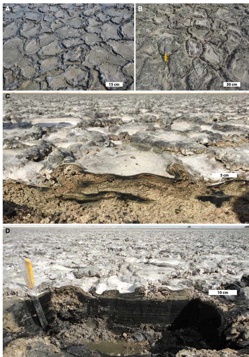
Fig. 3. Field photographs from the polygonal microbial mats. (A) Recently flooded polygons retaining water both within the polygons and in the inter-polygon gaps. (B) During low neap tides, the water within and between polygons may completely evaporate thus precipitating halite (the lighter colour within and between some polygons). The dashed line indicates the location of the cross-section in D. (C) A cross-section through polygons developed on a carbonate sand substrate, note the presence of two 'wispy' polygons within the sands. (D) A cross-section through microbial polygons developed over a substrate of planar-laminated microbial mats. Refer to Fig. 4 for a close up of the central polygon within this image.
