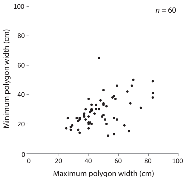
Fig. 2. A plot of the maximum polygon width (x-axis) against the minimum polygon width (y-axis).
