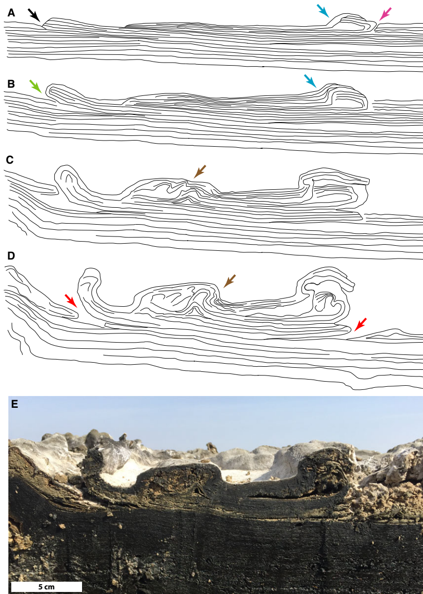
Fig. 4. A series of schematic diagrams showing the development of the microbial polygon shown in cross-section in E (see Fig. 3D for the context of this feature). (A) Optimum growth conditions result in displacive lateral growth of the microbial mats resulting in overthrusting (black arrow) and localized overturning (pink arrow) of the polygon margin. Continued microbial growth overgrows the margin to produce a rounded profile (blue arrow). (B) Continued laterally displacive growth increases overthrusting (green arrow) whilst vertical growth consolidates the margin (blue arrow). (C) As horizontal displacement continues, a new area of uplift is produced (brown arrow). (D) Polygon interior uplift continues (brown arrow). Increasing displacement at the polygon margins results in detachment of the polygon from the underlying substrate (red arrows) – the polygon is now susceptible to erosion. (E) Field photograph of a cross-section of a single microbial polygon.
