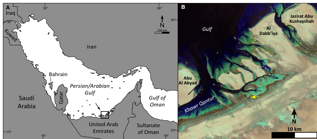
Fig. 1. (A) Map of the Gulf region (the arrowed box indicates the location of the satellite image in B). (B) Landsat Enhanced Thematic Mapper (ETM) image of the study area (acquired 3 July, 2002), see A for regional context. The location of the study area, in which the three transects were established, is indicated by the yellow arrow.
