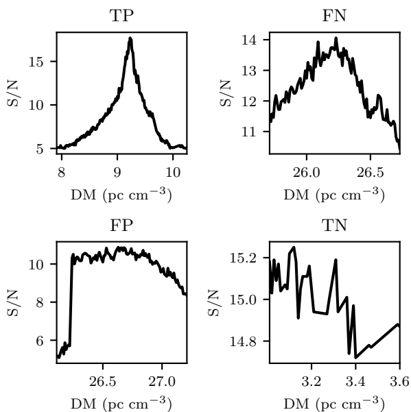
Figure 2. S/N curves along DM of four pulses with the relative classification indicated on top.
