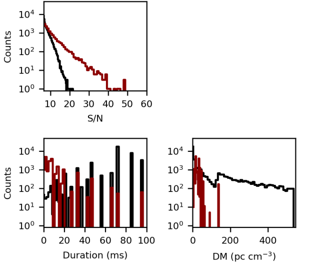
Figure 1. Comparison of the duration, S/N and DM of the RFI (black lines) and astrophysical (red lines) instances used in the LOTAAS training set.
