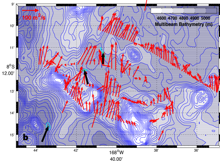
FIGURE 7. (a) P5 region \theta < 1^{\circ}\text{C} layer transport from multiple tow-yos and moorings during the 2014 Process cruise. Blue denotes the 50 m interval bathymetry contours. (b) Additional tow-yos from the same cruise give a magnified view (location in dashed box of panel a) of the flow around bumps and through gaps in the topographic structure near the sill. Several-day mooring averages (black arrows) match well with the tow-yo snapshot vectors, again indicating a dominantly steady flow direction and magnitude. Blue denotes the 25 m interval bathymetry contours.
