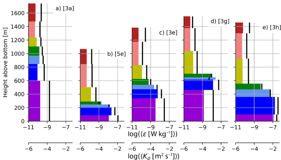
FIGURE 6. Comparison of turbulent kinetic energy dissipation ( \epsilon ) with diapycnal diffusivity ( K_\rho ) as a function of \Theta class for selected geographic groupings. Horizontal bars in each panel colored according to \Theta class show the average \epsilon and layer thickness (i.e., same as the panels in Figures 3 and 5). Vertical black lines give the average K_\rho in each \Theta layer. The number in square brackets in the upper-right corner of each panel corresponds to a panel in either Figure 3 or Figure 5. (a) Entrance to the eastern channel. (b) P3 sill. (c) P4 sill. (d) P5 sill. (e) Immediately downstream of the P5 sill.
