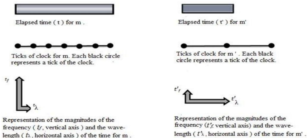
Figure 2. Schematic representation of time wavelength ( t_\lambda ) and time frequency ( t_f ) in relation to elapsed time and ticks of clock in relativistic speeds. Note that both t_\lambda and t_f have units of s^{-1} .
