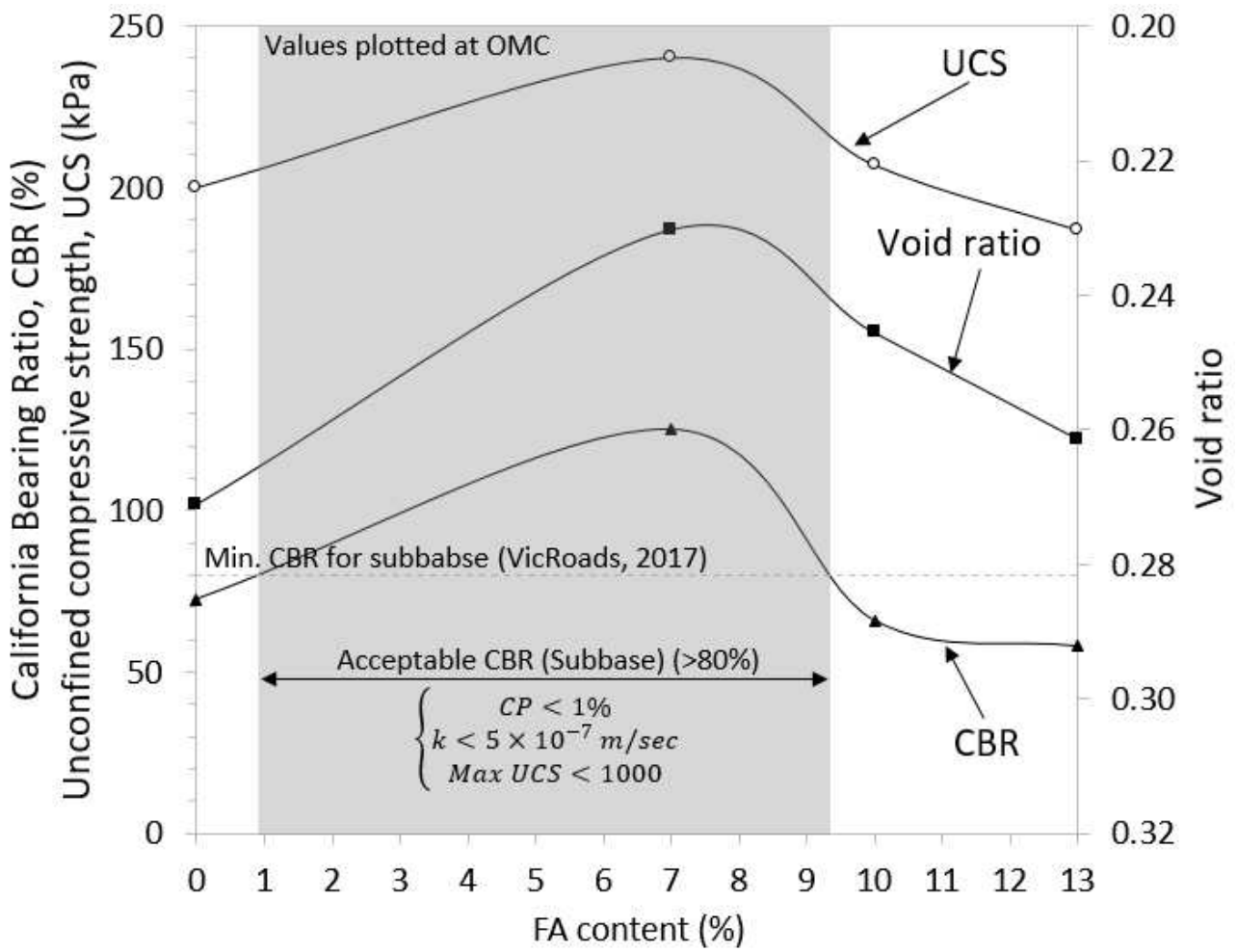
Figure 6: Variations of CBR, UCS and Void ratio under different FA content
