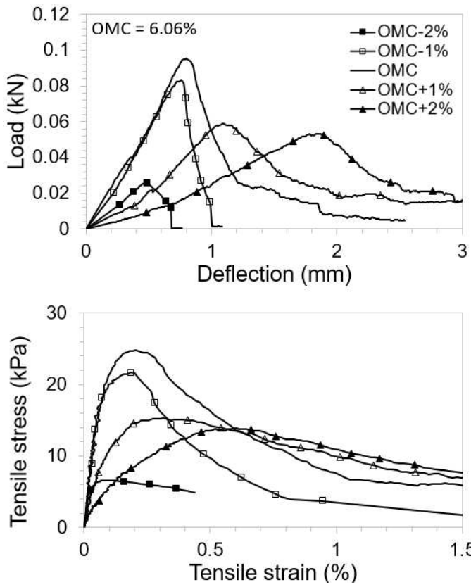
Figure 8: Tensile strength of CWFA mixture with 7% FA and different moisture contents
