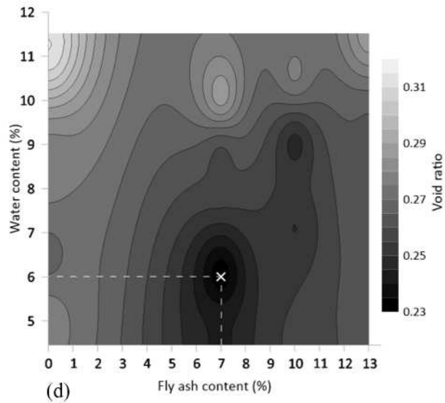
Figure 4: Compaction characteristics at (a-b) standard Proctor and (c-d) modified Proctor
