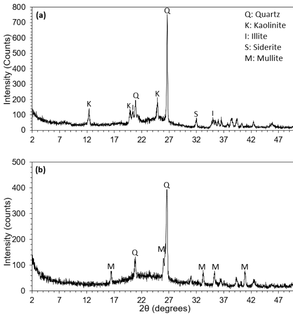
Figure 1: X-Ray diffraction of (a) coal wash and (b) fly ash
