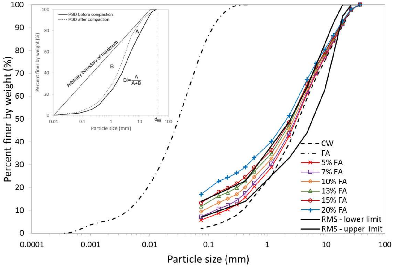
Figure 2: PSD curves of CW, FA and CWFA mixtures
