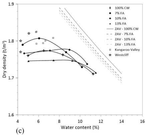
Figure 4: Compaction characteristics at (a-b) standard Proctor and (c-d) modified Proctor
