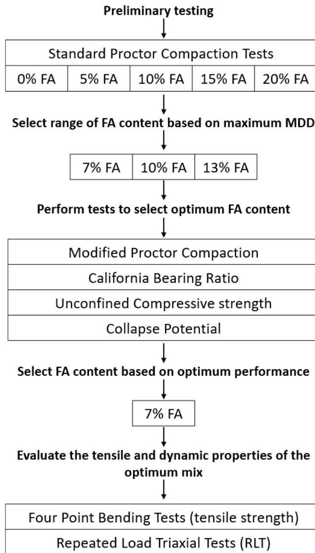
Figure 3: Schematic diagram of the experimental program followed to optimize the CWFA mixture
