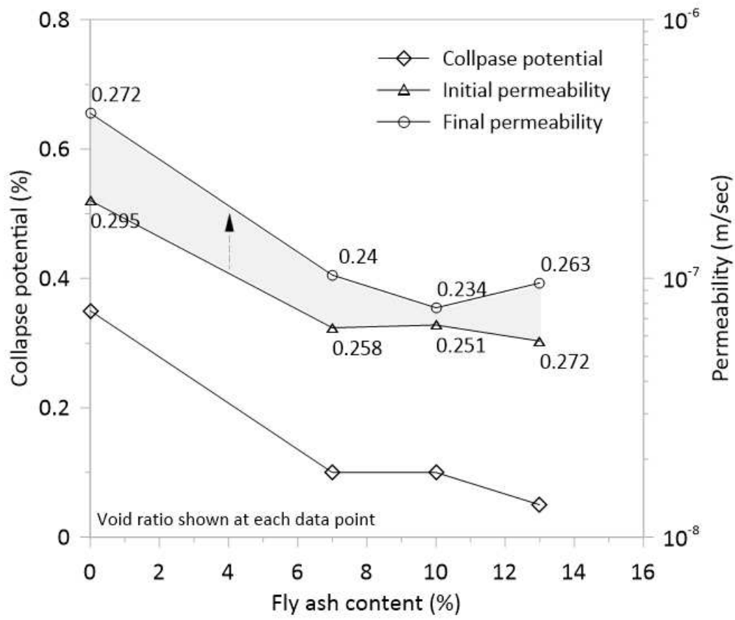
Figure 7: Collapse potential and associated change in permeability
