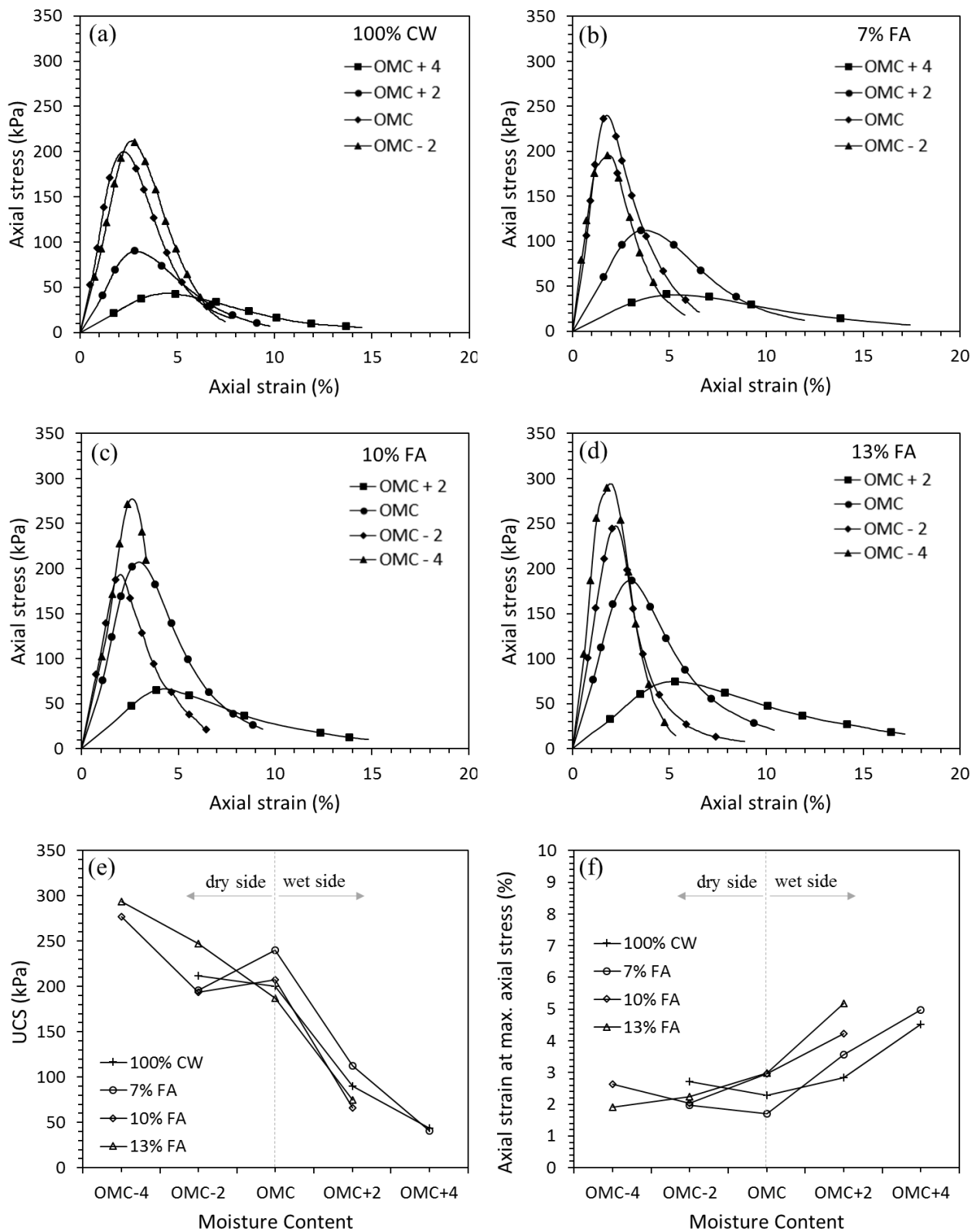
Figure 5: (a) Unconfined compressive strength of 100%CW, (b) Unconfined compressive strength of 7%FA, (c) Unconfined compressive strength of 10%FA, (d) Unconfined compressive strength of 13%FA, (e) variation of UCS with moisture, (f) variation of the axial strain at the maximum axial stress with moisture content
