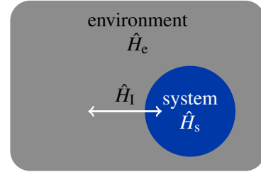
FIG. 7. System-bath interaction model where H_s , H_e , and H_1 are the system, environment, and interaction Hamiltonians.
