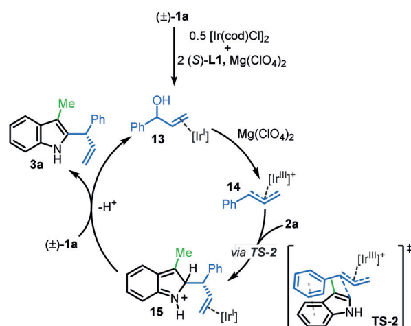
Scheme 6. Proposed mechanism.
