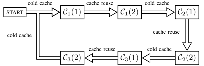
Fig. 2. Cache analysis of an example schedule (2, 2, 2) . After the first task \mathcal{C}_i(1) is executed, some instructions in the cache can be reused and thus the WCET of the following task is shortened.
