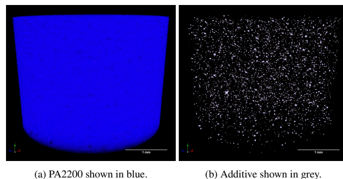
Figure 7: 3D views of 1.0% B65003 scan data.
