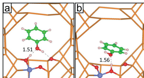
Fig. 7 (a) DFT-optimized structure and (b) snapshot of the DFT MD simulation after 7.5 ps of NVT simulation. The values of the H-bond distance Al-O-H \cdots O ph -H ph are shown for each structure ( \text{\AA} ). Colour code: Si (orange), O (red), Al (light blue), H (white) and C (green).
