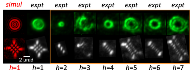
FIG. 7. Shown on top are the detailed structures of the diffracted beams and on the bottom their astigmatic transforms for a mask encoding \Phi_{21}^{TBB} . Here h is the order of diffraction, expt refers to data measured experimentally, and simul refers to theoretical simulation.
