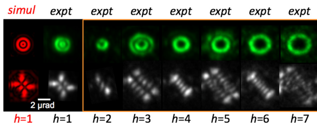
FIG. 6. Shown on top are the detailed structures of the diffracted beams and on the bottom their astigmatic transforms for a mask encoding \Phi_{11}^{TBB} . Here h is the order of diffraction, expt refers to data measured experimentally, and simul refers to theoretical simulation.
