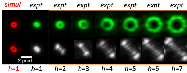
FIG. 5. Shown on top are the detailed structures of the diffracted beams and on the bottom their astigmatic transforms for the mask encoding \Phi_{01}^{TBB} . Here h is the order of diffraction, expt refers to data measured experimentally, and simul refers to theoretical simulation.
