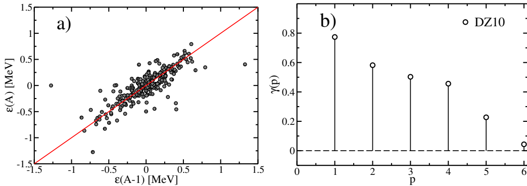
FIG. 2: (Colour online). Left panel: lag-plot of order 1 for DZ10 model. Right panel: evolution of the self-correlation coefficient defined in Eq.5 for different values of the lag. See text for details.
