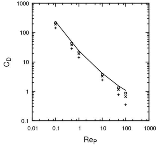
Figure 2: Simulated drag coefficient for icosphere face subdivisions, N_f , of 20 (+), 80 (x) and 320 ( \square ) compared against empirical values (—).
