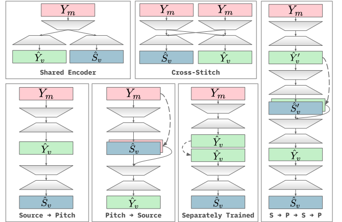
Fig. 5. Joint U-Net models. Each model takes the magnitude spectrogram of the mixture Y_m as input and outputs estimates of the vocal magnitude spectrogram \hat{Y}_v and the vocal f_0 salience \hat{S}_v . In Pitch → Source model, Y_m is given as additional input to the vocal source separation portion of the model (indicated by a dotted line), and similarly in the S → P → S → P model, the first vocal estimate \hat{Y}_v' is given as additional input to the second vocal source separation model. In Separately Trained , each network is trained separately, first optimizing \hat{Y}_v , and then using the optimized \hat{Y}_v as input to a second model that outputs \hat{S}_v .
