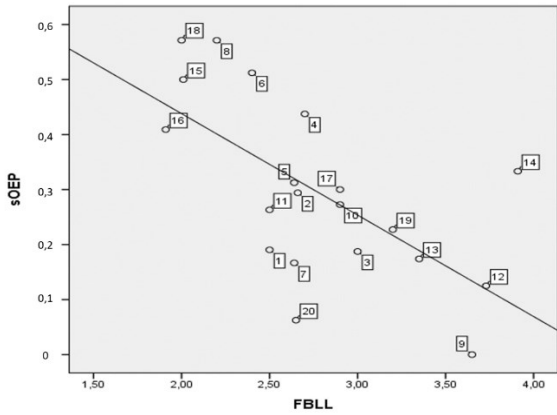
Figure 1a – Scatterplot and linear relationship between FBLL and sOEP in physical stores
