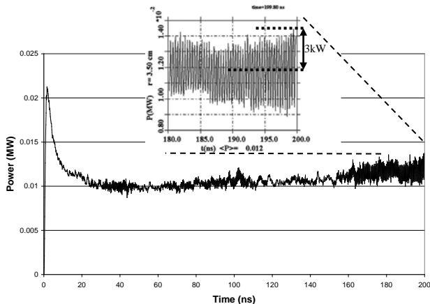
Fig. 4. Radial Poynting flux temporal evolution, measured in a plane at r = 3.5\text{cm} and spanning the length of the simulation.
