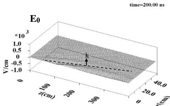
Fig. 3. 3D contour plot of E_{\theta} within an unbounded simulation geometry.
