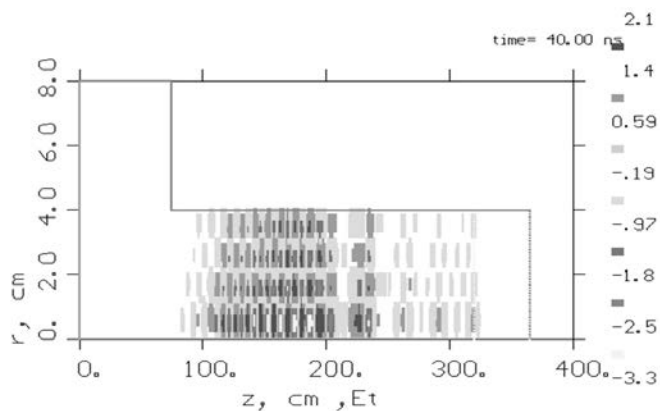
Fig. 2. Contour plot of E_\theta within a waveguide-bounded simulation geometry.
