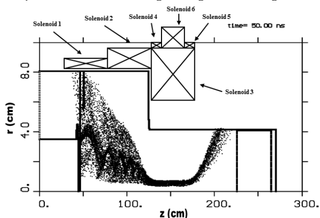
Fig. 1. Overview of experimentally consistent, waveguide-bounded PiC simulation geometry.
