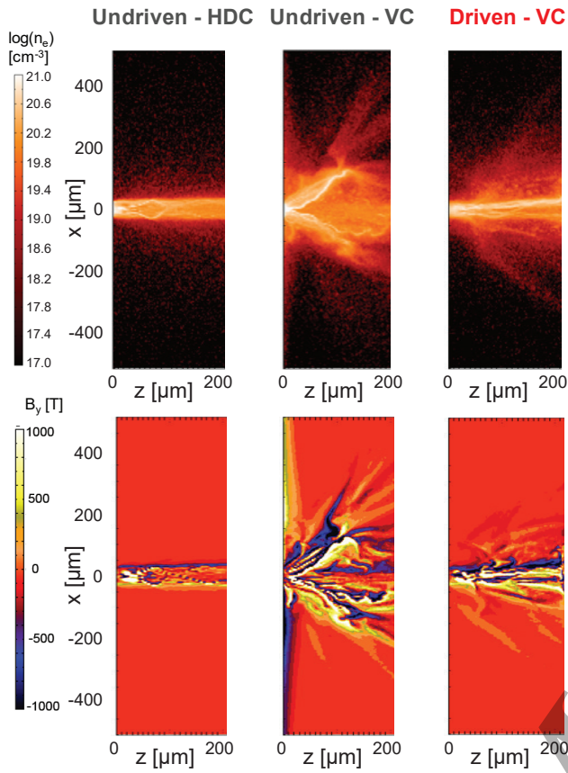
FIG. 7. Fast electron beam density (first row) and azimuthal self-generated magnetic field (second row) maps extracted from the REB transport simulations at t = 4 ps after the injection of the fast electrons, respectively for undriven diamond, undriven vitreous carbon and shock-heated vitreous carbon.
