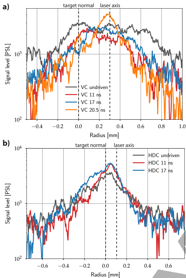
FIG. 3. K_{\alpha} lineouts along the radial direction from the SCI data for a) the VC cases (gray: undriven, red: \Delta t = 11 ns, blue: \Delta t = 17 ns, orange: \Delta t = 20.5 ns) and for b) the diamond cases (gray: undriven, red: \Delta t = 11 ns, blue: \Delta t = 17 ns).
