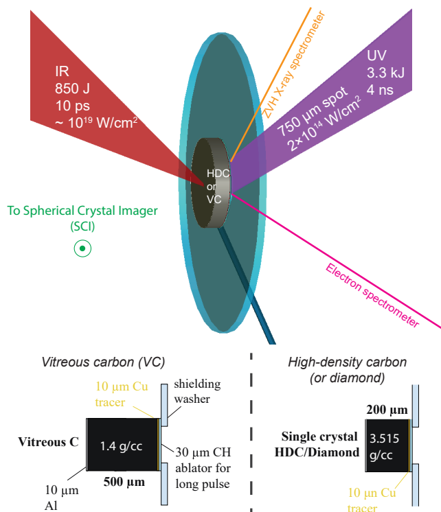
FIG. 1. Sketch of the experimental setup from the spherical imager's (SCI) line-of-sight. The relativistic electron beam (REB) is generated by the intense 10 ps laser, focused onto the center of the front surface of a carbon cylinder of 3 mm diameter made of vitreous carbon (VC) or diamond (HDC) with the same initial \rho R of 70 \text{ mg/cm}^3 .
