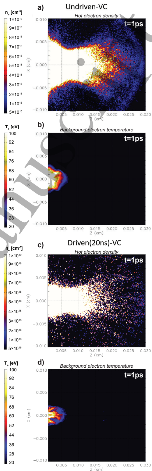
FIG. 6. Hot electron density [a)-c)] and background electron temperature [b)-d)], respectively for undriven VC and driven VC ( \Delta t = 20.5 ns) at 1 ps after the REB injection.
