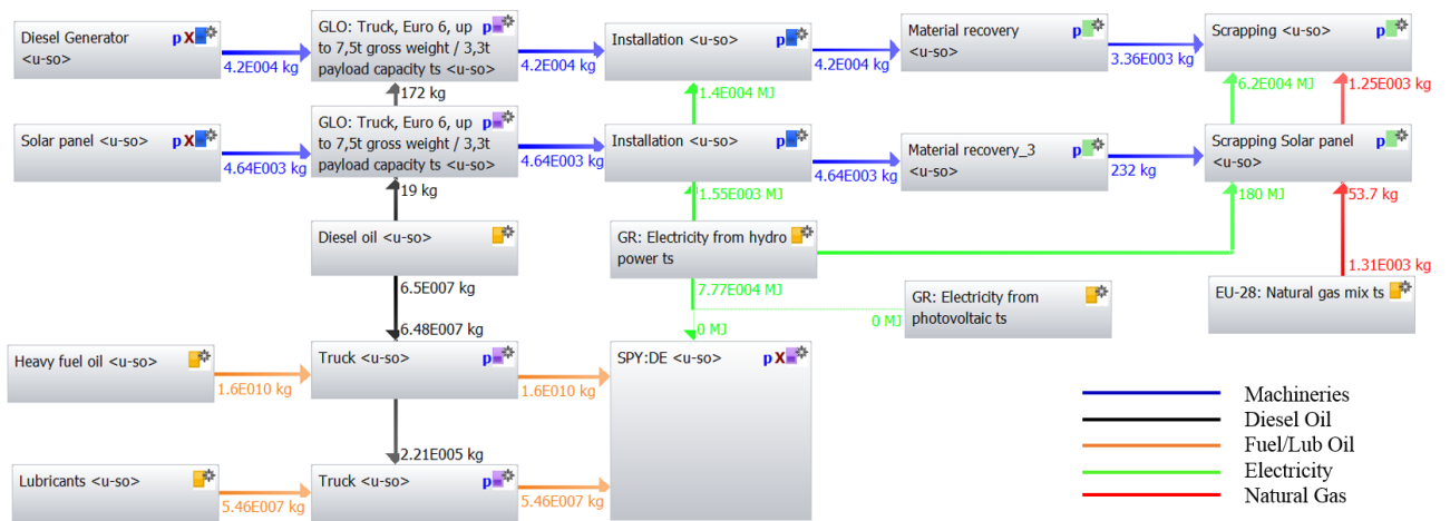
Figure 6 Flowchart of LCA processes in GaBi
