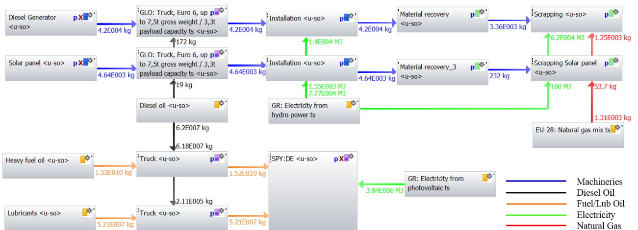
Figure 7 LCA analysis flowchart of Scenario 2: with solar panel application
