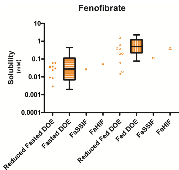
Fig. 10. Design of experiment equilibrium solubility measurements. Legend: Equilibrium solubility measurements for Fenofibrate in DOE media compositions detailed in Table 1. Solubility values found in reduced fasted DOE shown as ●, reported solubility values found in original fasted DOE shown as [14], reported solubility values found in fasted simulated intestinal fluid shown as [3], reported solubility values in fasted human intestinal fluid shown as ▲ [3], solubility values found in reduced fed DOE shown as ○ solubility values found in original Fed DOE shown as [14] reported solubility values found in fed intestinal simulated fluid shown as [14] and reported solubility values found in fed human intestinal fluid shown as ▲.
