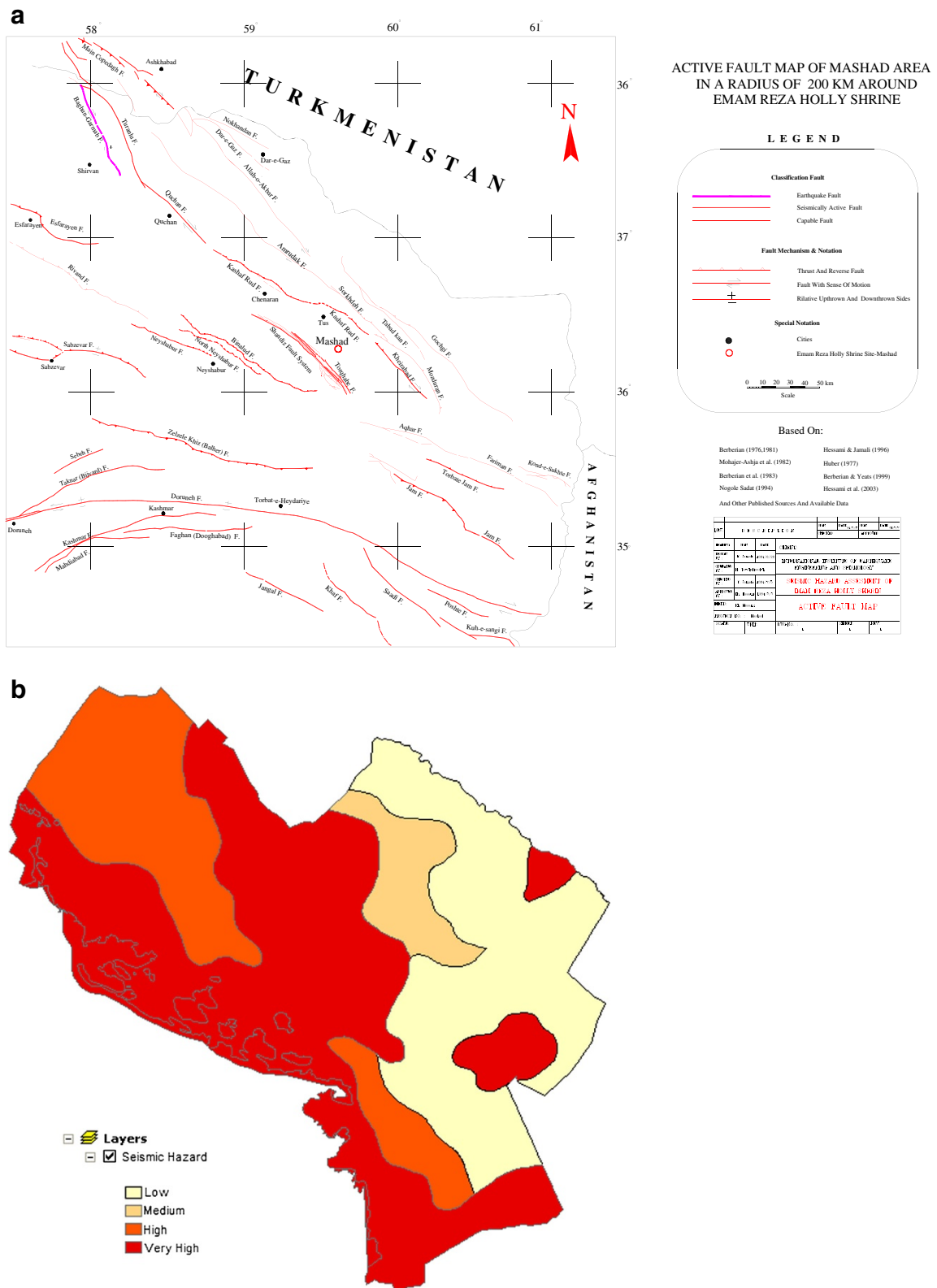
Figure 1 Regional seismology of the Mashhad city: (a) active faults and (b) seismic hazard map. Adapted from Hafezi-Moghaddas (2007).
