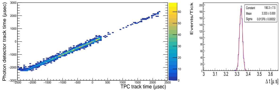
Figure 5.25: PD system timing measurements: Correlation between the TPC and the PD system track time (left); time difference between two consecutive calibration flashes, demonstrating a resolution of 14 ns (right).
