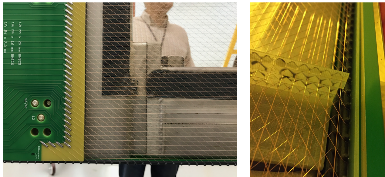
Figure 2.13: Left: APA corner where end boards meet side boards. The injection molded teeth that guide the U and V wires around the edge are visible at the bottom. Right: The wire support combs.
