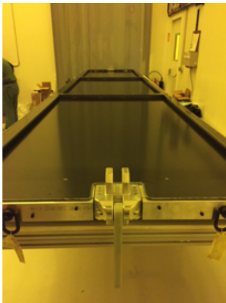
Figure 1.8: A ProtoDUNE-SP cathode plane assembly. The black surface is the carbon-impregnated Krypton resistive cathode plane.
