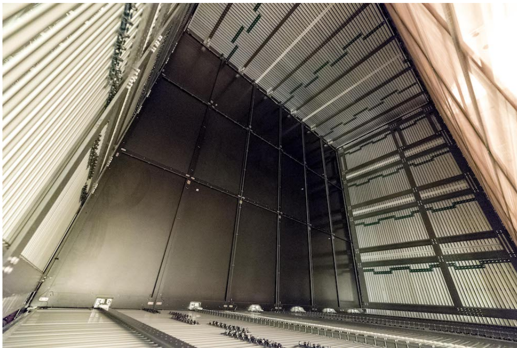
Figure 3.18: One of the two drift volumes of ProtoDUNE-SP. The FC modules shown enclose the drift volume between the CPA array (at the center of the image) and the APA array (upper right). The endwall FCs are oriented vertically; the top and bottom units are horizontal. The staggered printed circuit boards connecting the endwall FC profiles are the voltage divider boards.
