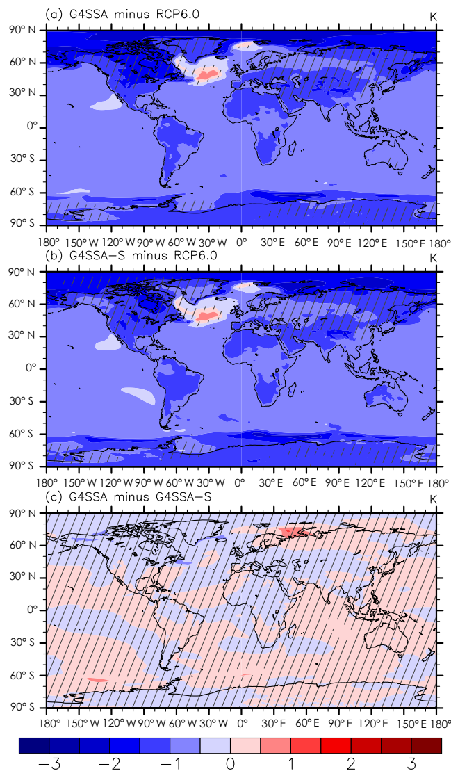
Figure 3. Global maps of surface temperature differences (K) between (a) G4SSA and RCP6.0, (b) G4SSA-S and RCP6.0, and (c) G4SSA and G4SSA-S over the period 2030–2069. Hatched regions are areas with p > 0.05 (where changes are not statistically significant based on a paired t test).
