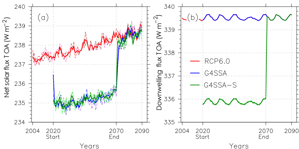
Figure 1. (a) Global averaged annual net solar flux at the top of the atmosphere ( \text{W m}^{-2} ) and (b) downwelling solar flux at the top of the atmosphere ( \text{W m}^{-2} ). Dashed lines are ensemble members, and solid lines are the average of three ensemble members. Geoengineering starts on 1 January 2020 and ends on 1 January 2070. The 11-year periodicity is imposed as a prediction of the sunspot cycle. In (b) the G4SSA curve exactly covers the RCP6.0 curve.
