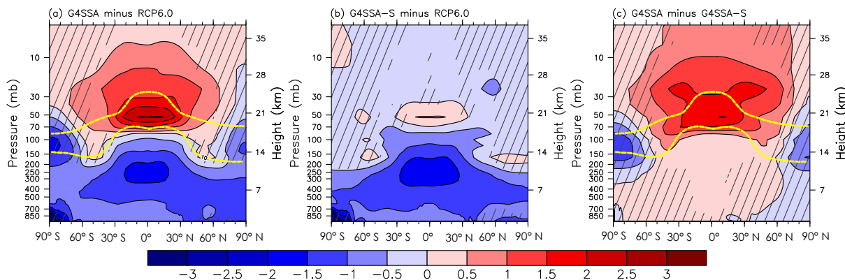
Figure 4. Zonal mean temperature differences (K) in the geoengineering experiments (a) G4SSA minus RCP6.0, (b) G4SSA-S minus RCP6.0, and (c) G4SSA minus G4SSA-S. These are averaged for the three ensemble members for the years 2030–2069. Hatched regions are insignificant, with p > 0.05 . The yellow dashed lines in (a) and (c) are upper and lower limits of the prescribed sulfate aerosol (surface area density: 10 \mu\text{m}^2 \text{cm}^{-3} ).
