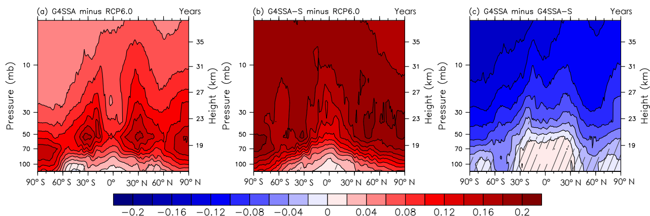
Figure 9. Zonal mean age of air differences (years) between (a) G4SSA and RCP6.0, (b) G4SSA-S and RCP6.0, and (c) G4SSA and G4SSA-S. They are averaged for the three ensemble members for 2030–2069. Hatched regions are insignificant, with p > 0.05 .
