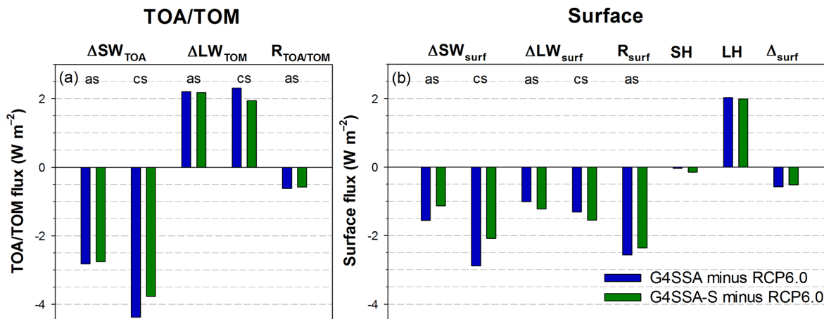
Figure 5. Energy flux (a) the top of the atmosphere (TOA)/the top of the model (TOM) (b) and at the surface (surf), shown as G4SSA minus RCP6.0 and G4SSA-S minus RCP6.0 for 2030–2069. For all fluxes, downwelling is positive. \Delta SW is the net shortwave flux, \Delta LW is the net longwave flux, R is the sum of \Delta SW and \Delta LW , SH is sensible heat, LH is latent heat, and \Delta_{surf} is the sum of \Delta SW_{surf} , \Delta LW_{surf} , SH , and LH ; as is all sky and cs is clear sky.
