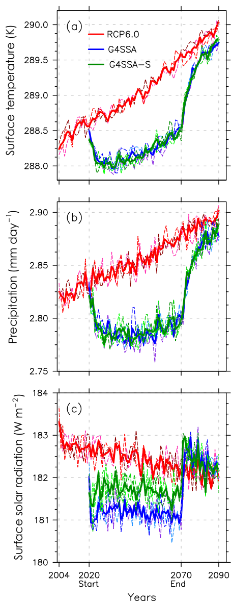
Figure 2. (a) Global averaged annual surface air temperature (K), (b) global averaged annual precipitation ( \text{mm day}^{-1} ), and (c) downwelling surface solar radiation ( \text{W m}^{-2} ). Dashed lines are ensemble members, and solid lines are the average of the three ensemble members. Geoengineering starts on 1 January 2020 and ends on 1 January 2070.
