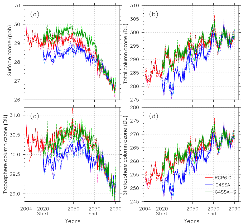
Figure 6. (a) Global averaged annual surface ozone concentrations (ppb), (b) total column ozone (DU), (c) tropospheric column ozone (DU), and (d) stratospheric column ozone (DU). An ozone concentration of 150 ppb is used as the boundary of tropospheric ozone and stratospheric ozone. Dashed lines are ensemble members, and solid lines are the average of the three ensemble members. Geoengineering starts on 1 January 2020 and ends on 1 January 2070.
