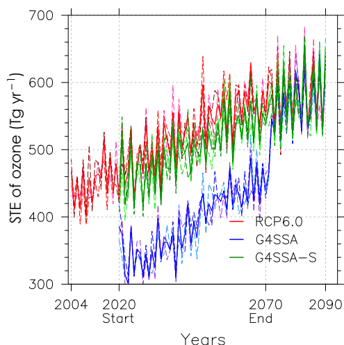
Figure 10. Global annual averaged ozone transported from the stratosphere to the troposphere (STE of ozone) in \text{Tg yr}^{-1} . Geoengineering starts on 1 January 2020 and ends on 1 January 2070.
