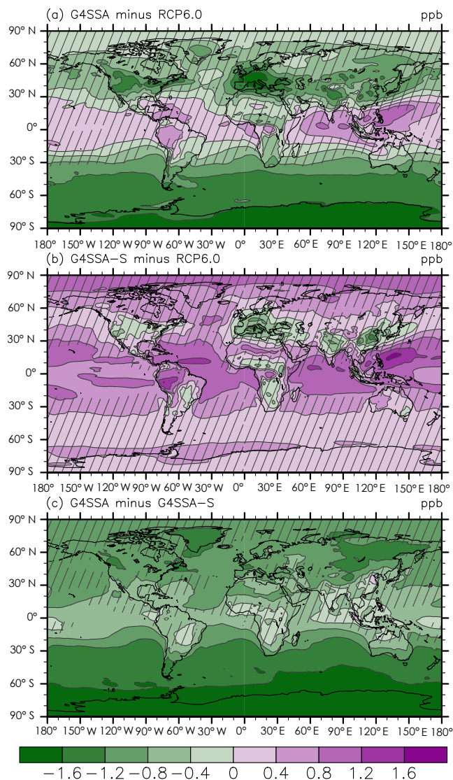
Figure 7. Global maps of surface ozone concentration differences (ppb) between (a) G4SSA and RCP6.0, (b) G4SSA-S and RCP6.0, and (c) G4SSA and G4SSA-S for 2030–2069. Hatched regions are insignificant, with p > 0.05 .
