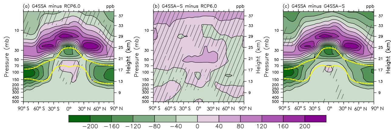
Figure 8. Zonal mean ozone concentration differences (ppb) in the geoeengineering experiments, averaged for the three ensemble members for 2030–2069. Hatched regions are insignificant, with p > 0.05 . The yellow dashed lines in (a) and (c) are the upper and lower limits of the prescribed sulfate aerosol (surface area density: 10 \mu\text{m}^2 \text{cm}^{-3} ).
