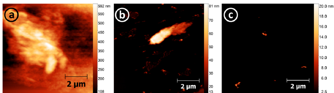
Figure 8. Atomic force microscopy (AFM) typical morphologies of aggregated A \beta_{25-35} in the presence or absence of HCO _4^- (two-electron oxidant) or CO _3^{\bullet-} (one-electron oxidant) after 24 h aggregation. The aggregated amyloid (a) sample present almost everywhere amorphous structures and globular aggregates of several microns in size. The one-electron reaction (b) sample is similar to the aggregated one in terms of dimensions of the aggregates but their presence is diminished. Two-electron oxidation sample (c), instead, present smaller and scattered structures of elongated nature, in this latter sample very rarely were observed amorphous structures of several hundreds of nanometers in size.
