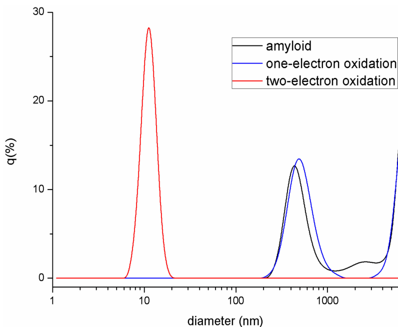
Figure 11. Dynamic light scattering (DLS) analyses of A\beta_{25-35} in the presence or absence of HCO_4^- (two-electron oxidant) or CO_3^{\bullet-} (one-electron oxidant). Only the sulfoxide formation (red line) mediated by HCO_4^- stops the aggregation process at nano-scale level.
