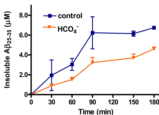
Figure 10. \text{A}\beta_{25-35} aggregation in the presence or absence of peroxymonocarbonate. Reaction mixture contained 10 \mu\text{M} \text{A}\beta_{25-35} in 0.1 \text{ M} phosphate buffer, pH 7.4, and 0.1 \text{ mM} DTPA (squares), when present, peroxymonocarbonate was added at 0.8 \text{ mM} final concentration (triangles). After various time incubation at 37^\circ\text{C} , the reaction was stopped by addition of catalase ( 400 \text{ U/mL} ) and the reaction products analyzed by HPLC.
