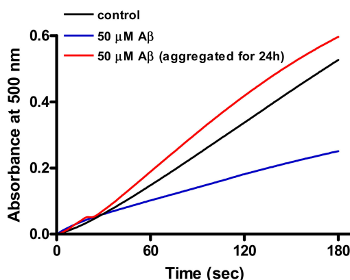
Figure 7. Effect of different aggregation states on the reaction rate of DHR oxidation by CO 3 •- . Freshly dissolved A \beta_{25-35} (blue line) and aggregated A \beta_{25-35} (red line) after 24 h incubation. A \beta_{25-35} (50 \mu\text{M} final concentration) was added to a solution containing 25 \mu\text{M} DHR, 31 \mu\text{M} SOD, 0.1 mM DTPA, and 25 mM sodium bicarbonate in 0.2 M phosphate buffer, pH 7.4. Reaction was started by the addition of 1 mM H 2 O 2 . DHR oxidation rate was measured spectrophotometrically at 500 nm.
