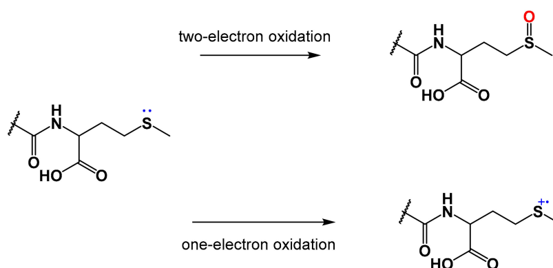
Scheme 1. One- and two-electron oxidations of A\beta_{25-35} methionine residue on the thioether sulfur.
