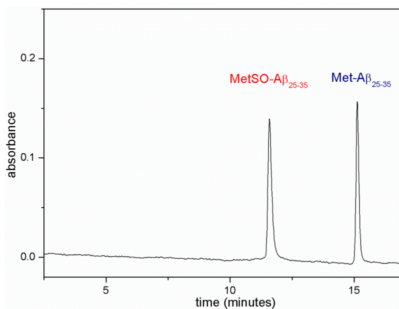
Figure 1. HPLC profile of A\beta_{25-35} incubated for 120 min with peroxymonocarbonate (PMC or HCO_4^- ). 10 \mu\text{M} A\beta_{25-35} was allowed to react with peroxymonocarbonate at 0.8 \text{ mM} final concentration in 0.1 \text{ M} phosphate buffer, pH 7.4, containing 0.1 \text{ mM} DTPA. After 120 min at room temperature, aliquots of incubation mixture were analyzed by HPLC.
