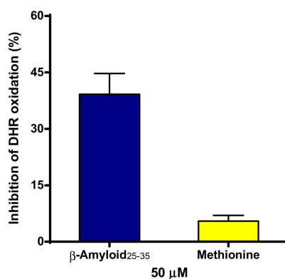
Figure 6. Effect of A \beta_{25-35} and L-Met on DHR oxidation mediated by carbonate radical anion. A \beta_{25-35} or L-methionine (50 \mu\text{M} final concentration) was added to a solution containing 25 \mu\text{M} DHR, 31 \mu\text{M} SOD, 0.1 mM DTPA, and 25 mM sodium bicarbonate in 0.2 M phosphate buffer, pH 7.4. Reaction was started by the addition of 1 mM H 2 O 2 . Oxidized DHR was quantified spectrophotometrically at 500 nm.
