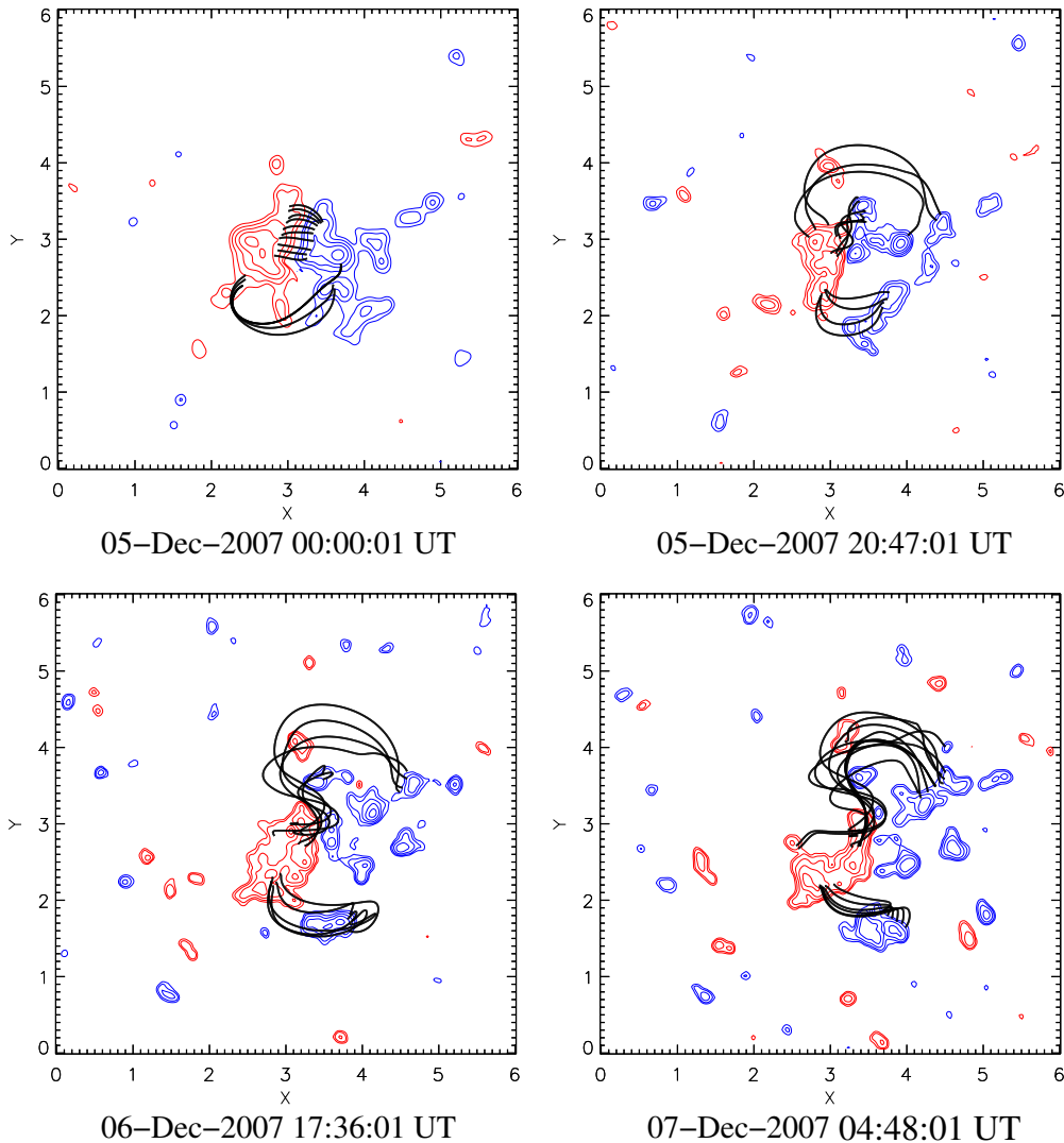
Figure 7. Field line plots generated from the simulation at various times approximately corresponding to the times in Figure 2. The red and blue contours denote the positive and negative photospheric fields, respectively.
