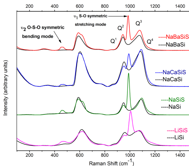
Figure 2. Raman spectra of the \text{SO}_3 -free and \text{SO}_3 -doped silicate glasses.
