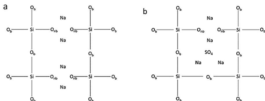
Figure 12. Schematic showing the repolymerizing effect of SO 3 incorporation on a silicate network. (a) Fragment of the silicate network containing two units of Na 2 O, showing the connectivity of the bridging (O b ) and non-bridging (O nb ) oxygen atoms. The incorporation of each unit of Na 2 O converts one O b to two O nb . (b) Same fragment of the silicate network after the addition of one unit of SO 3 . The sulfur atom is at the center of a SO 4 group, directly bonded only to sodium atoms. The formation of the SO 4 group leads to the conversion of two O nb to one O b . Note that these diagrams are intended to show only the connectivity of the atoms but not to convey information about the distances between atoms.
