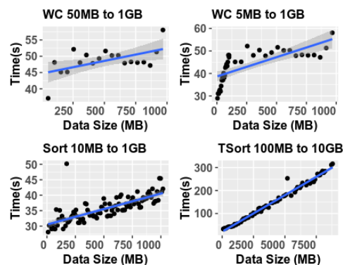
Fig. 1: Execution time for varying datasets for MapReduce WordCount, TeraSort and Simple-Sort Programs
