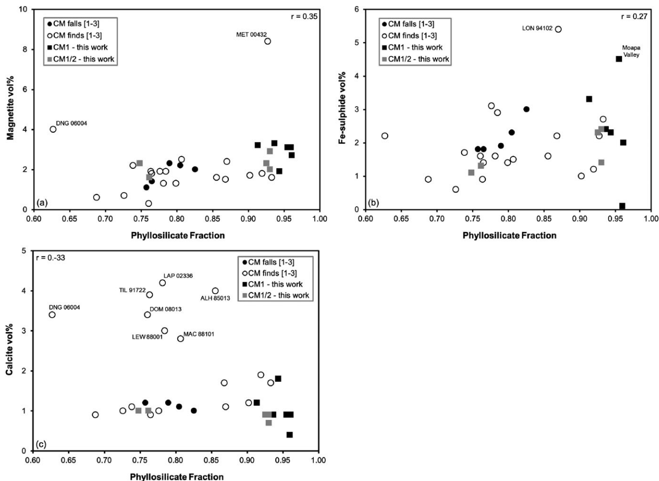
Fig. 4. Variations in the abundance of (a) magnetite, (b) Fe-sulphide, and (c) calcite with increasing aqueous alteration in the CM chondrites. The degree of alteration is determined from the phyllosilicate fraction (total phyllosilicate abundance/[total anhydrous silicate + total phyllosilicate abundance], see text for details). Data for 21 CM2, 1 CM1/2, and 2 CM1 chondrites (falls and finds) are taken from [1] Howard et al. (2009), [2] Howard et al. (2011a), and [3] Howard et al. (2015).
