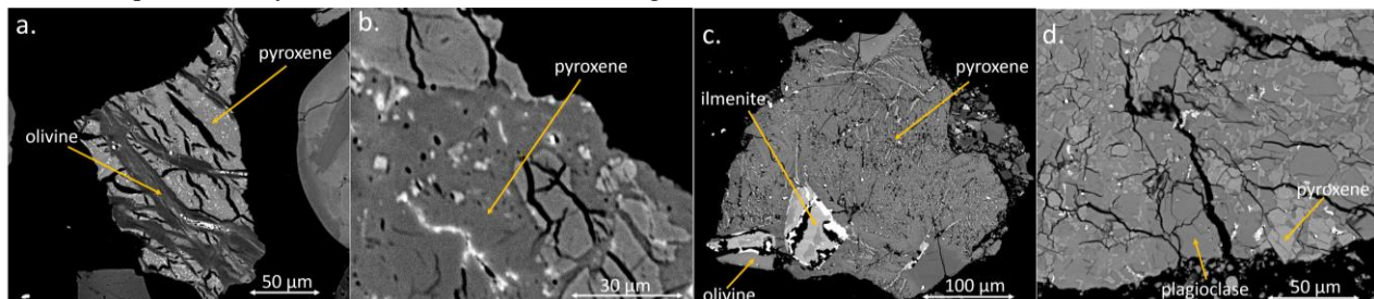
Fig. 2 Example BSE images from the reacted materials. Bright white blebs indicating Fe formation are identified in all samples. a.) NU-LHT-2M, b.) NWA12592, c.) 10084, and d.) 60500.
