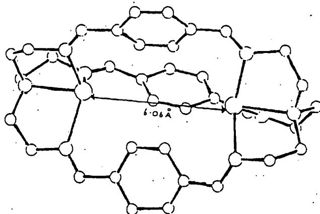
Figure 38 The X-ray crystal structure of \text{Ag}_2\text{3Bp}(\text{CF}_3\text{SO}_3)_2
