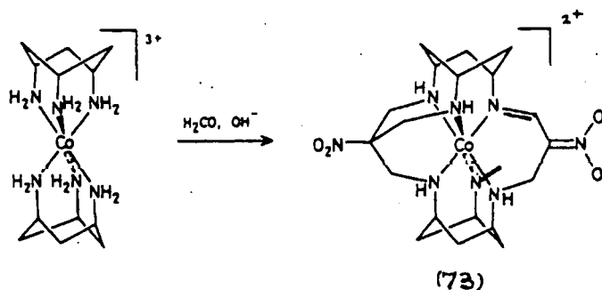
Scheme 22
