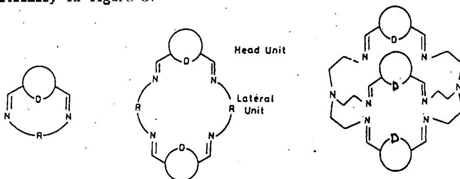
Figure 5 Schematic representations of 1+1, 2+2 and 2+3 Schiff-base ligands
