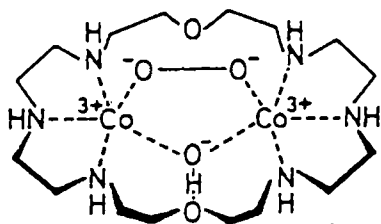
\mu -Hydroxo- \mu -peroxo-dicobalt bisdien chelate
