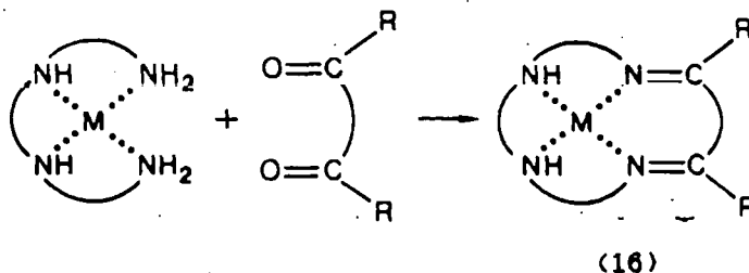
Scheme 9
