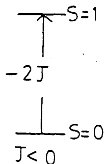
Antiferromagnetic
