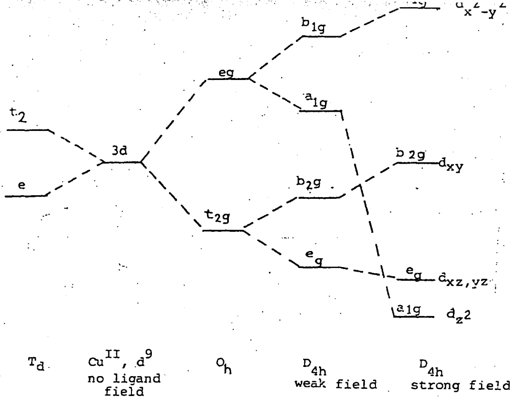
Figure 49 d-orbital splitting for Cu(II) in T_d , O_h and D_{4h} symmetries
