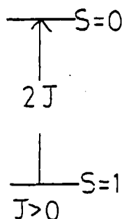
Ferromagnetic
