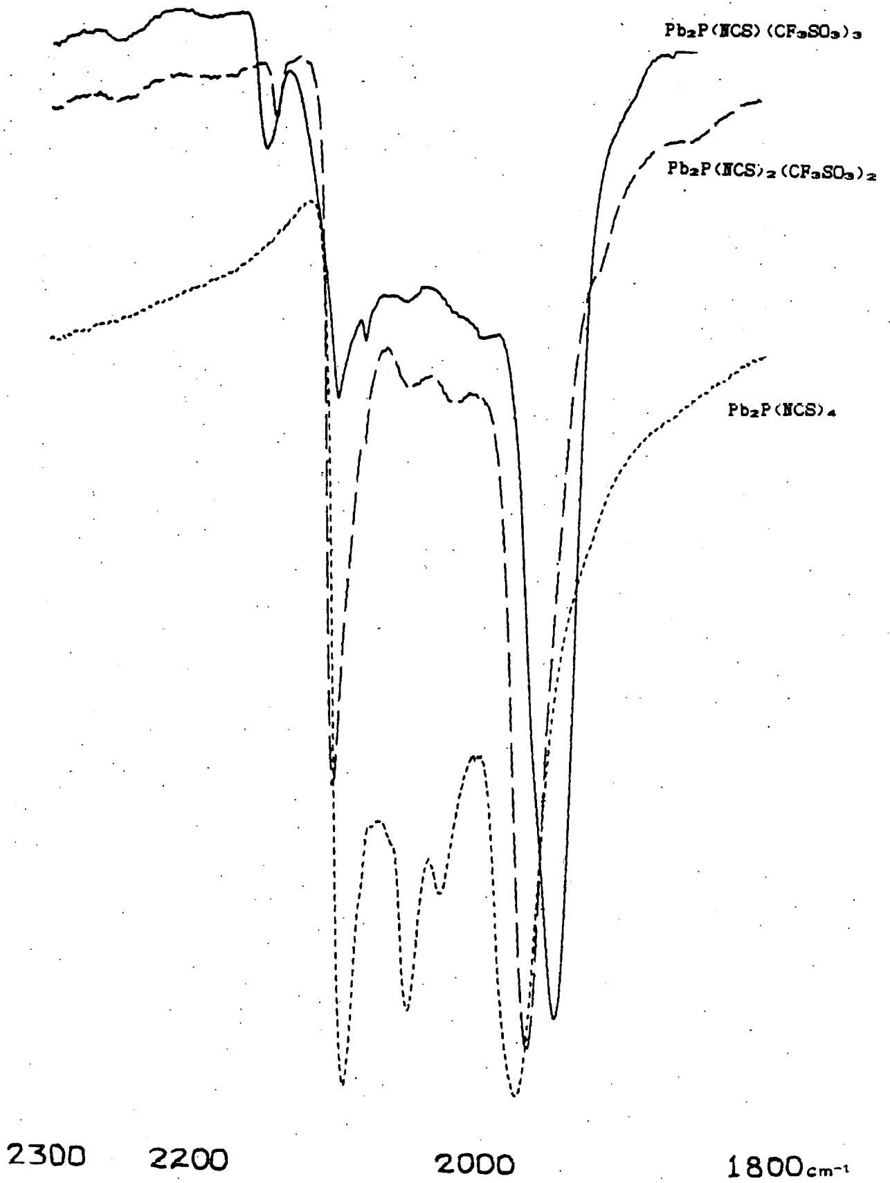
Figure 9 The \nu_{\text{as}}(\text{NCS}) stretching region of dilead P thiocyanates
