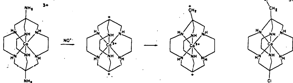
Scheme 25 Formation of the absar cage by rearrangement
