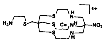
Scheme 24
