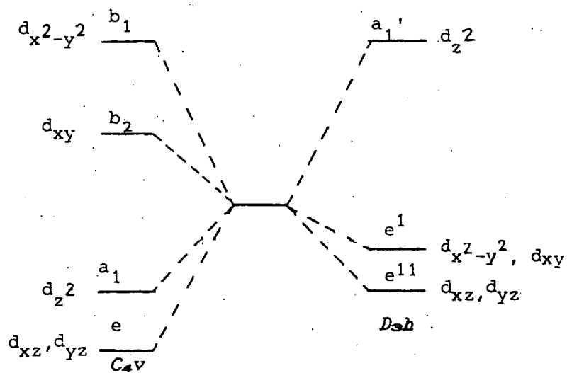
Figure 50 d-orbital splitting for Cu(II) in C_{4v} and D_{3h} symmetries
