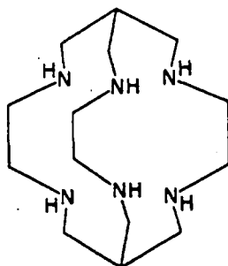
(65) Sarcophagine
