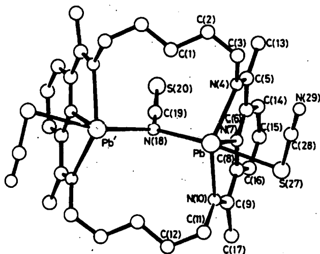
Figure 8 The X-ray crystal structure of \text{Pb}_2\text{P}(\text{NCS})_4
