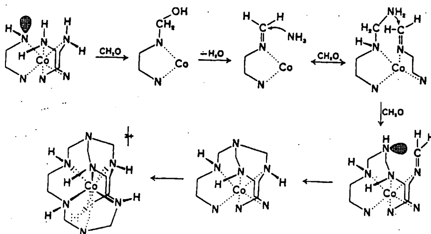
Scheme 18 Proposed synthesis of [\text{Co(III)Sepulchrato}]^{3+} ion
