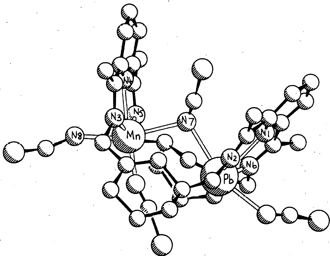
Figure 22 The X-ray structure of \text{MnPb}_2\text{NC}(\text{NCS})_4 .
