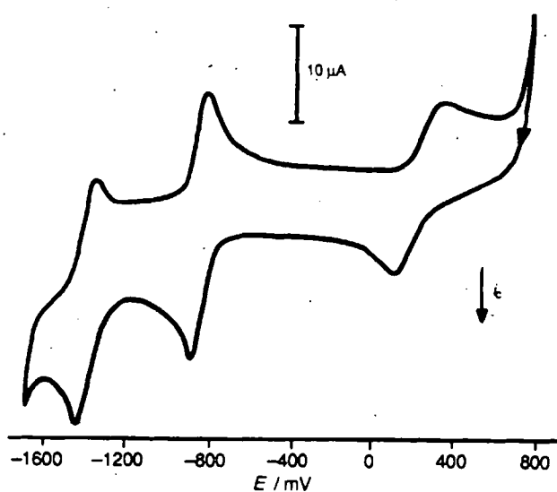
Figure 34 The cyclic voltammogram of CoGT(BPh 4 ) 2 in dmf;
