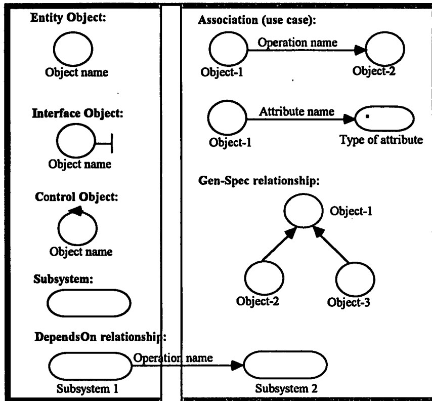
Figure 2.2 OOSE Notation
