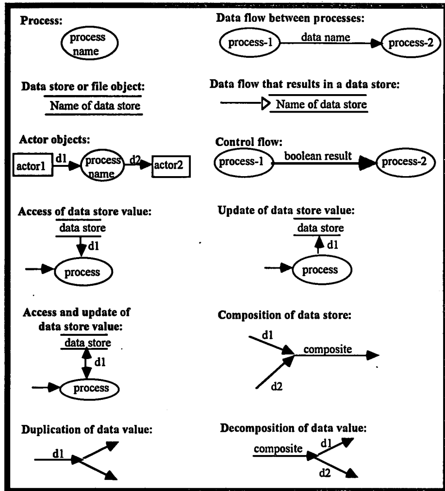
Figure 4.6 The Symbols in Data Flow Diagrams
