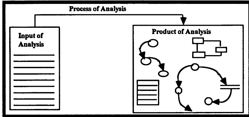
Figure 3.4 Object-Oriented Analysis
