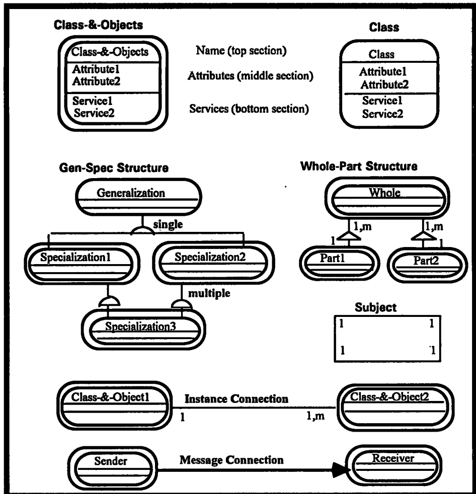
Figure 4.1 OOA Notation
